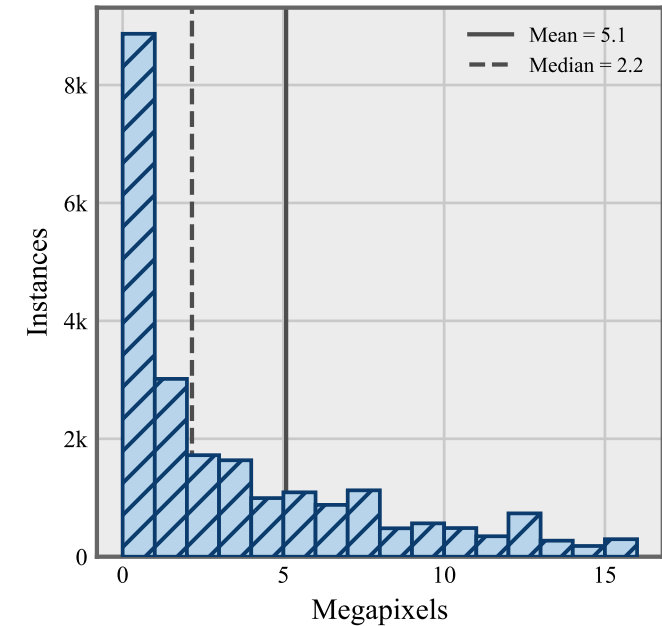
Image resolution
