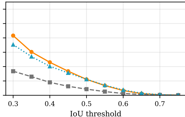
CADICA (out-of-distribution)
