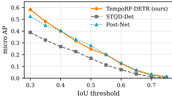
RIPCID-test (in-distribution)
