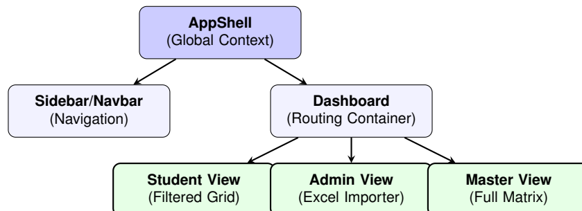
FIGURE 5.8: Hierarchical Structure of the Core React Components
