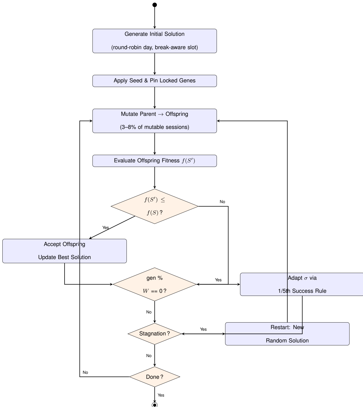
FIGURE 5.2: Activity Diagram: (1+1)-ES Solver Execution Flow
