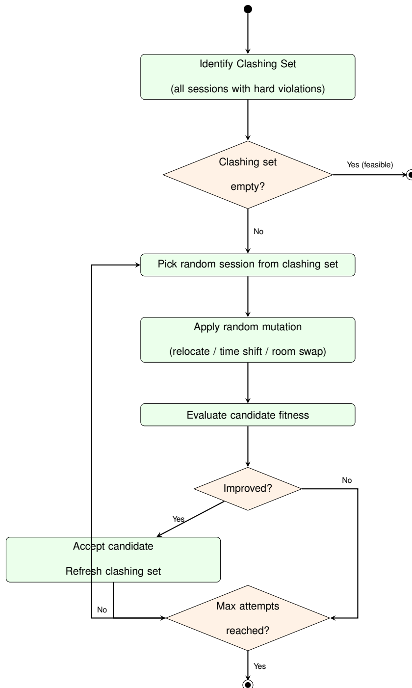
FIGURE 5.3: Activity Diagram: LNS Destroy-and-Repair Auto-Fix
