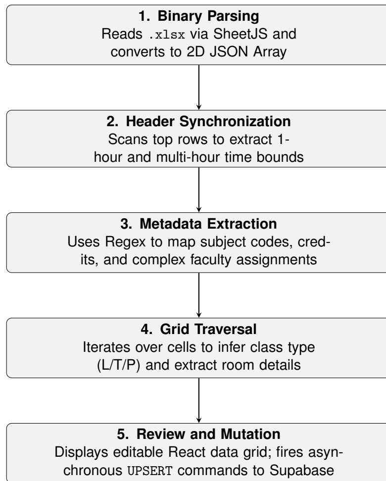
FIGURE 4.3: Data Ingestion Pipeline for Excel Timetables
