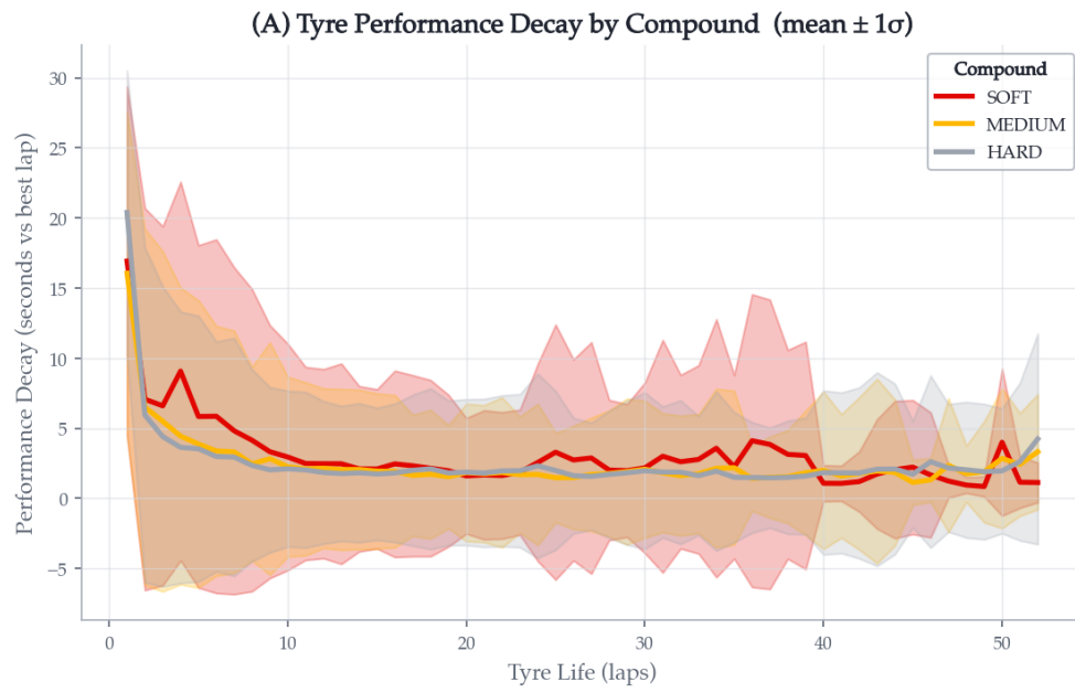
Figure 31. Compound-specific tyre degradation curves: mean performance loss (seconds vs. best lap) as a function of tyre age, with \pm 1\sigma band. All three compounds collapse rapidly over the first five laps; Soft shows the highest sustained mean decay and the widest variance band.
