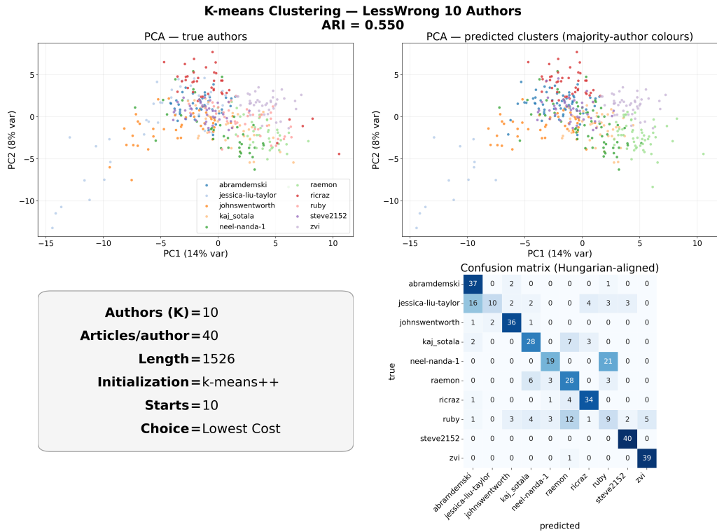
Figure 1: K-means on the LessWrong 10 Authors dataset, K = 10 . Top left: articles projected onto the two PCA directions of largest variance ( sklearn.decomposition.PCA applied to the centered, z-scored matrix), coloured by true author. Top right: same projection, coloured by predicted cluster (each cluster takes the colour of its majority author). Bottom right: confusion matrix after a Hungarian one-to-one alignment ( scipy.optimize.linear_sum_assignment ) between predicted clusters and true authors.
