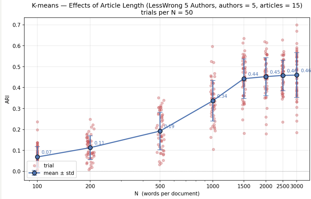
Figure 8: ARI vs. N on LessWrong 5 Authors ( K = 5 , M = 15 , 50 trials per N ). The curve follows the 10-author trend up to N = 1500 , then flattens : ARI moves only from 0.44 to 0.46 over the range N \in \{1500, 2000, 2500, 3000\} .
