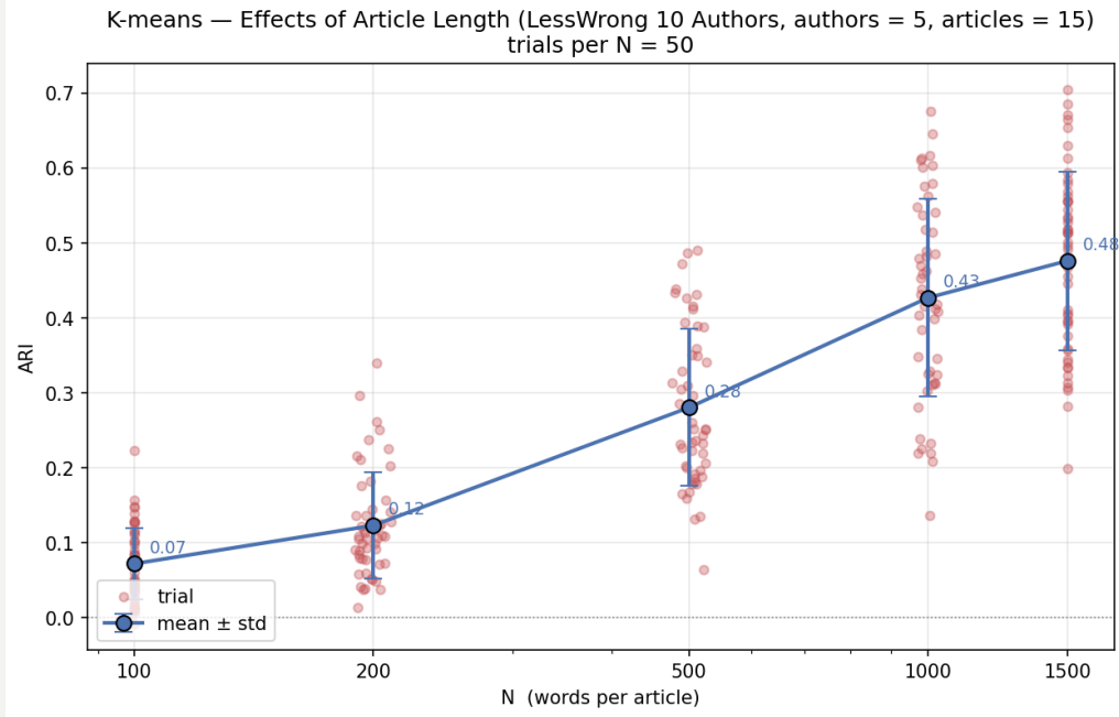
Figure 7: ARI vs. N on LessWrong 10 Authors ( K = 5 , M = 15 , 50 trials per N ). ARI rises steeply from 0.07 at N = 100 to 0.48 at N = 1500 .
