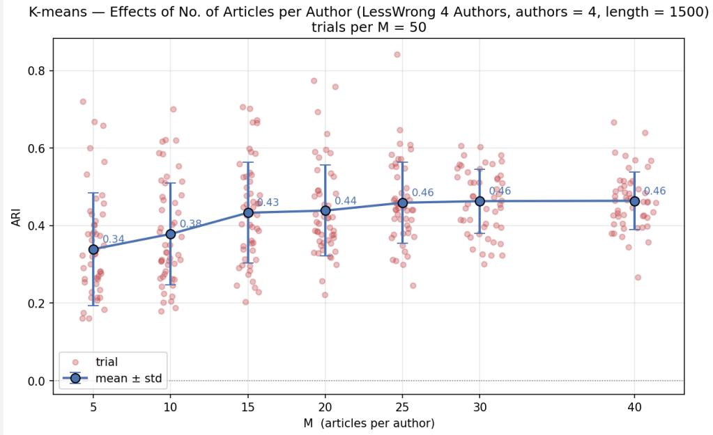
Figure 5: ARI vs. M on LessWrong 4 Authors ( K = 4 , N = 1500 , 50 trials per M ). The curve climbs from 0.34 at M = 5 to \sim 0.46 near M = 25 , then plateaus through M = 40 .
