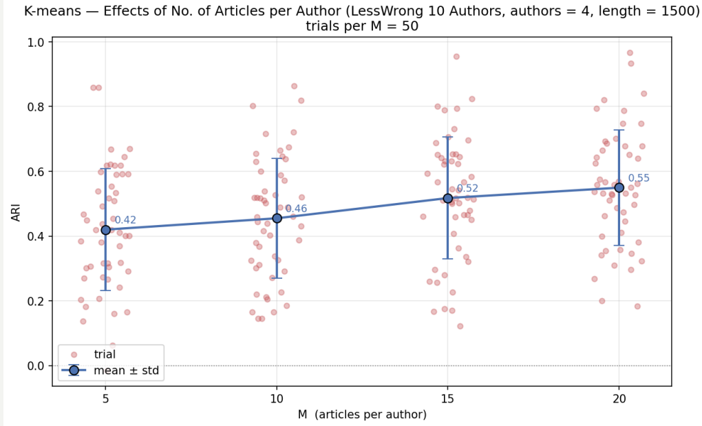
Figure 4: ARI vs. M on LessWrong 10 Authors ( K = 4 , N = 1500 , 50 trials per M ). Mean ARI rises from 0.42 at M = 5 to 0.55 at M = 20 .
