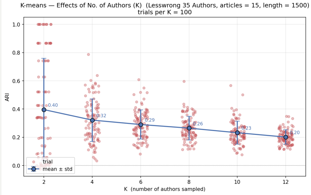
Figure 6: ARI vs. K on LessWrong 35 Authors ( M = 15 , N = 1500 , 100 trials per K ). Mean ARI falls monotonically from 0.40 at K = 2 to 0.20 at K = 12 . The spread shrinks rapidly with K .
