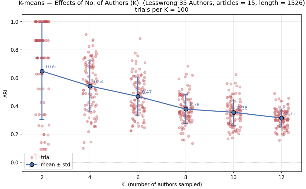
Figure 7: ARI vs. K on LessWrong 35 Authors ( M = 15 , N = 1526 , 100 trials per K ). Mean ARI falls monotonically from 0.65 at K = 2 to 0.31 at K = 12 . The spread shrinks rapidly with K .
