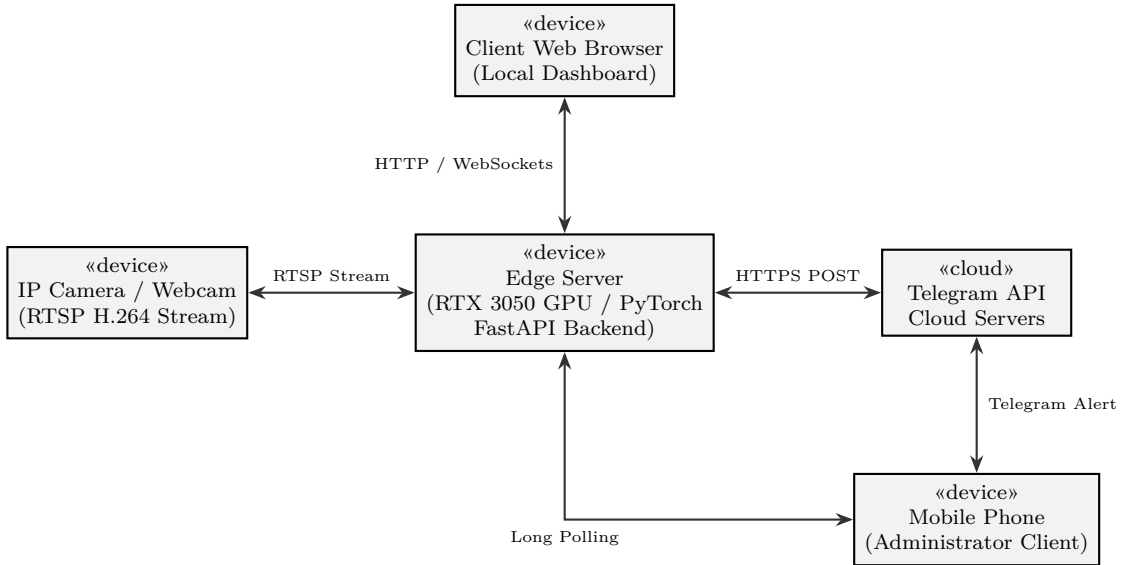
Figure 5: System Hardware and Software Deployment Diagram
