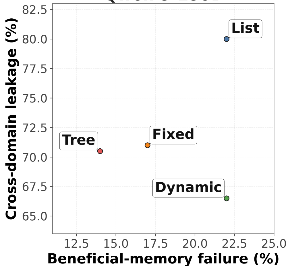
Qwen 3-235B
