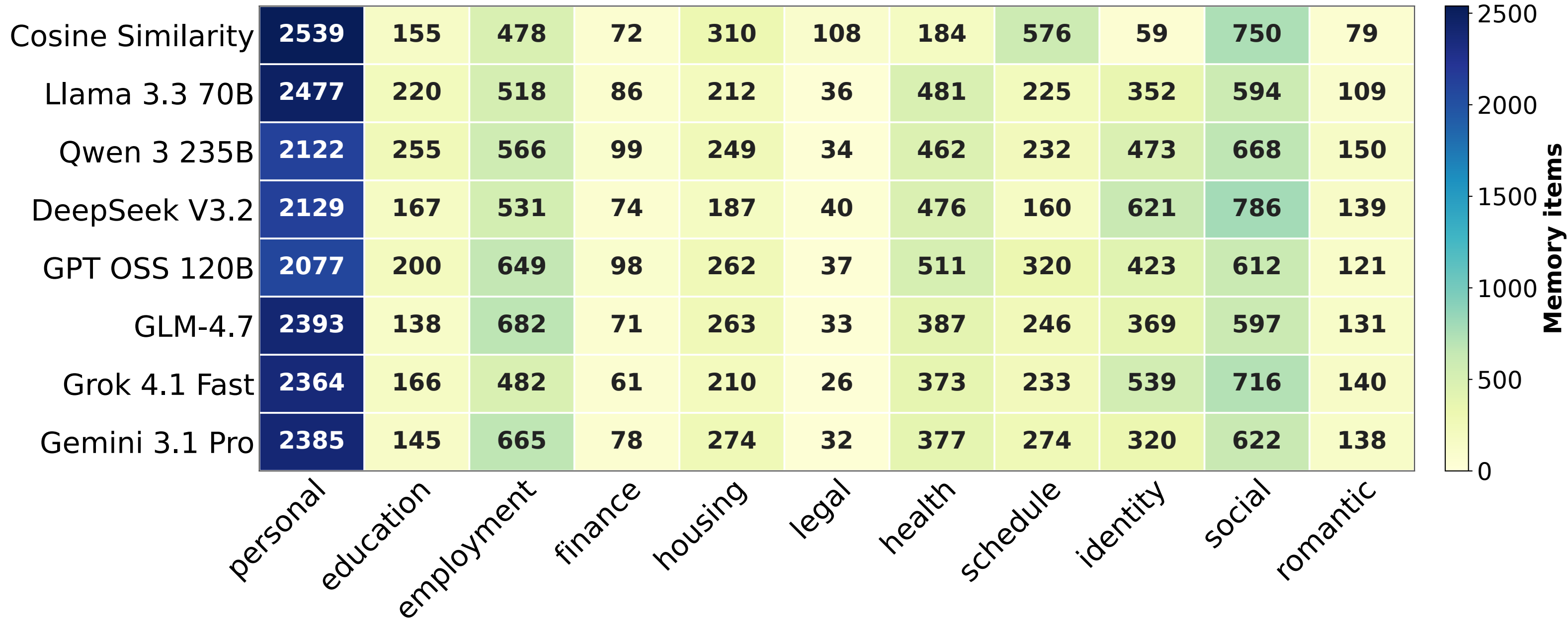
Memory Distribution of Inference and Cosine Similarity Fixed Partitions
