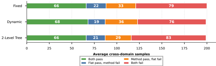
Cross-Domain Overlap vs. Flat: Model Average
