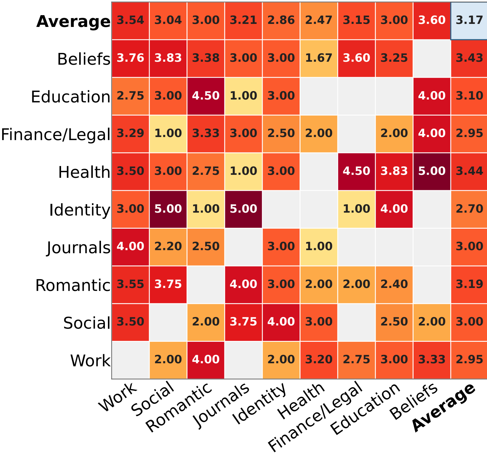
2-Level Tree
