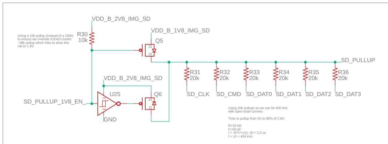
SD Pullup Voltage Switching (2.8V <-> 1.8V)
