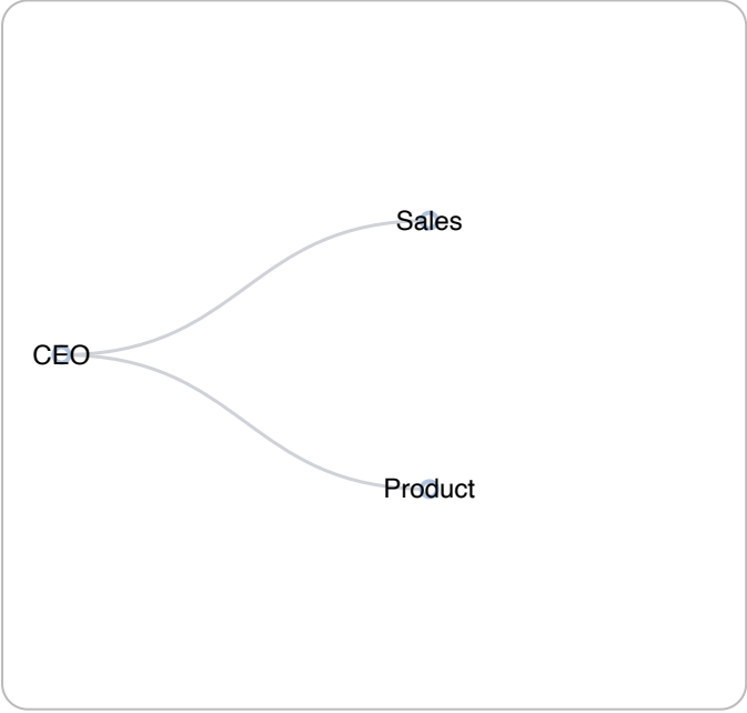
tree
