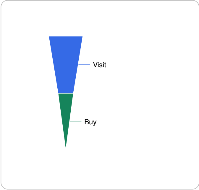
funnel
