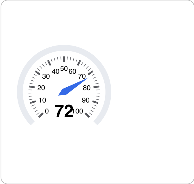
gauge
