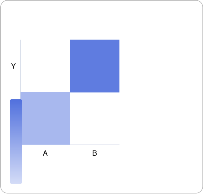
heatmap
