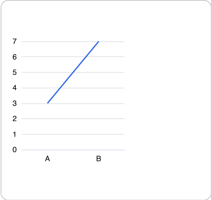
line
