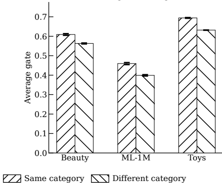
(b) Target-related gate
