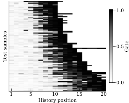
(a) Gate heatmap
