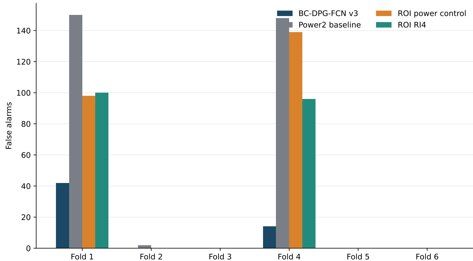
Fold-level false alarms at frozen thresholds
