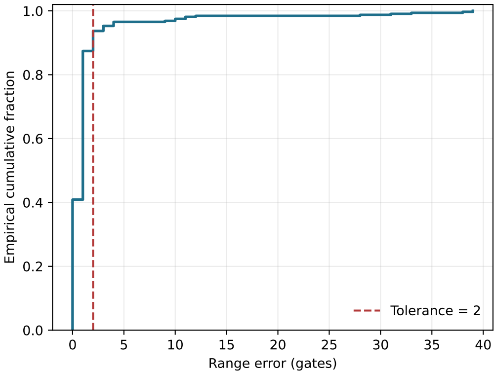
BC-DPG frozen six-fold target localization errors
