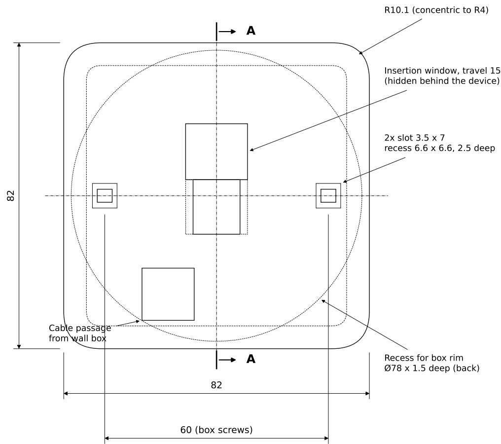
Wall plate for flush wall box, front view
