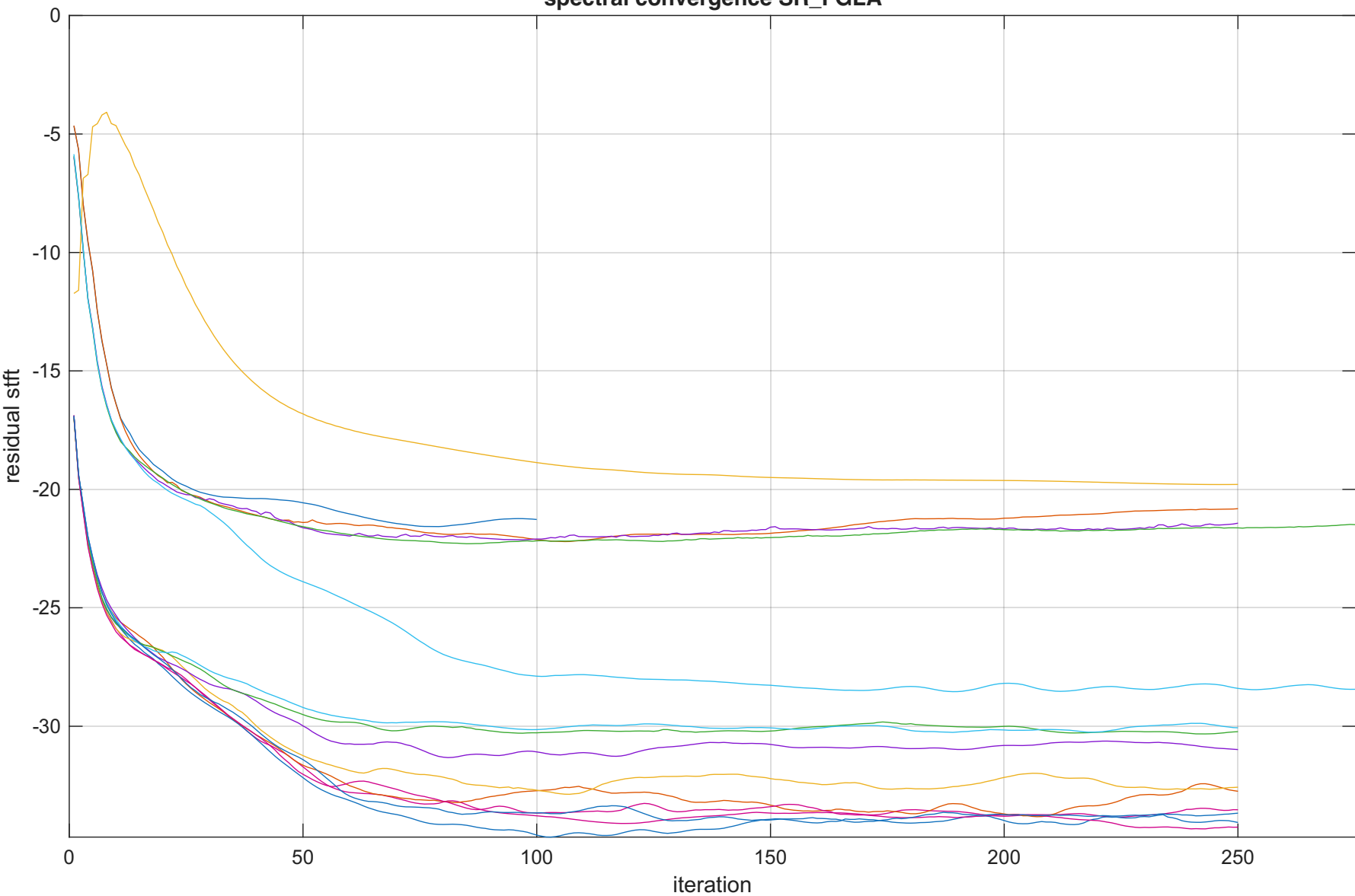
spectral convergence SR_FGLA
