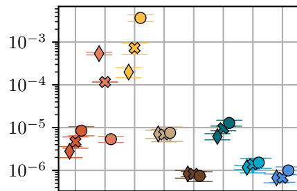
Lorenz, Pred: 13
