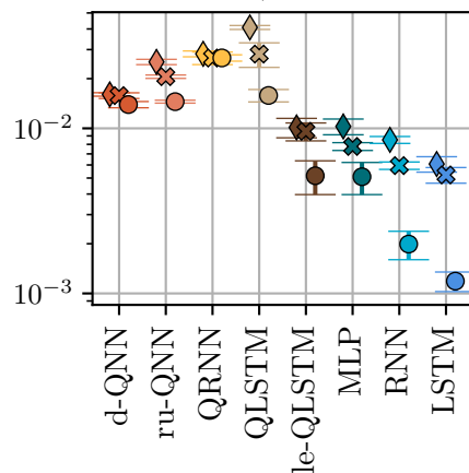
Lorenz, Pred: 25
