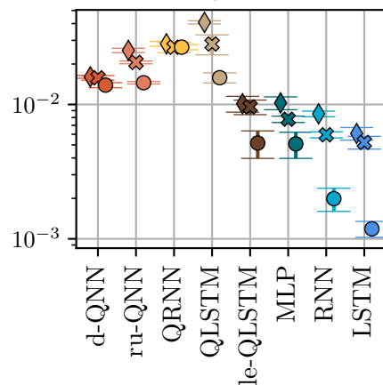
Lorenz, Pred: 25
