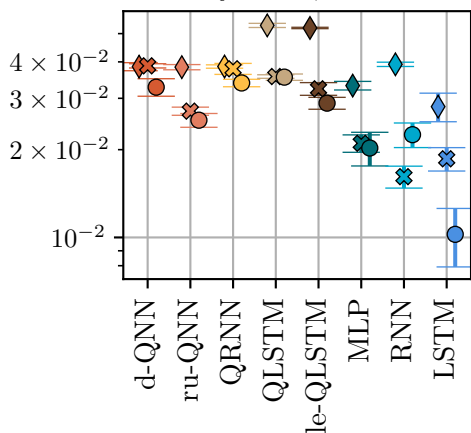
Mackey-Glass, Pred: 140
