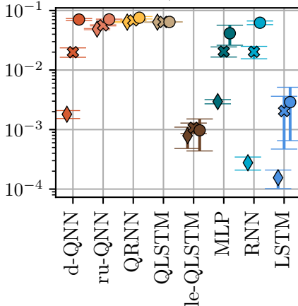
Hénon, Pred: 4
