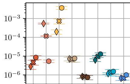
Lorenz, Pred: 13
