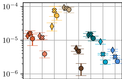
Mackey-Glass, Pred: 70
