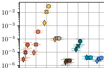
Hénon, Pred: 2
