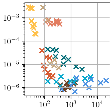
Seq: 4, Pred: 13
