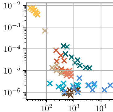
Seq: 16, Pred: 13
