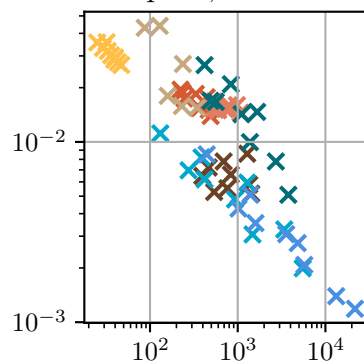
Seq: 16, Pred: 25
