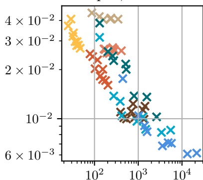
Seq: 4, Pred: 25
