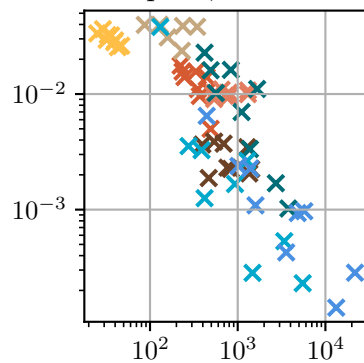
Seq: 16, Pred: 25
