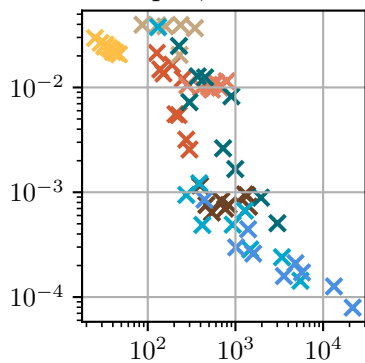
Seq: 8, Pred: 25
