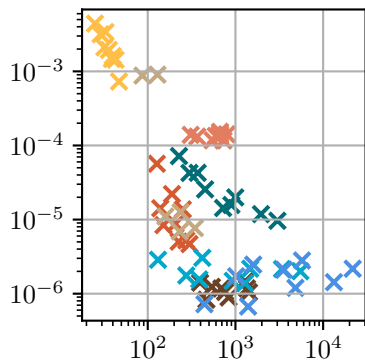
Seq: 8, Pred: 13
