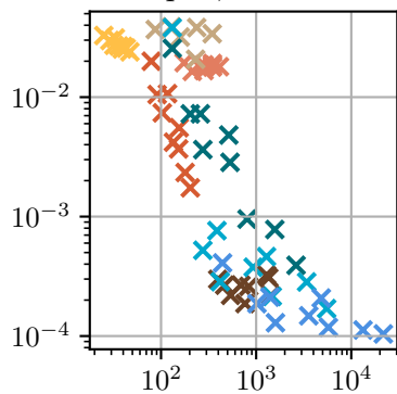
Seq: 4, Pred: 25
