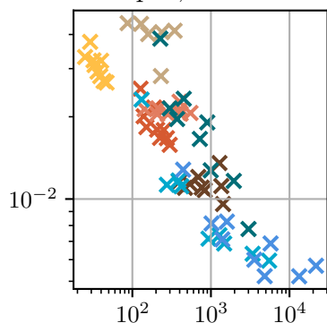
Seq: 8, Pred: 25
