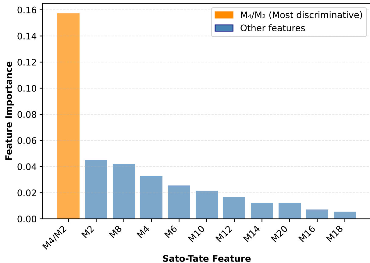
b) Sato-Tate Moments &amp; Ratios
