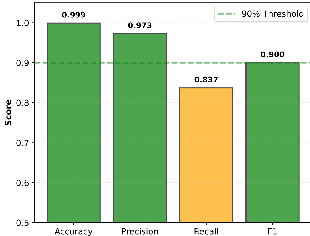
Classification Metrics (5-fold CV)
