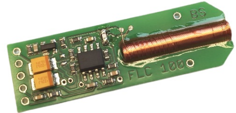
(b) Fluxgatemagnetometer FLC100 [26]
