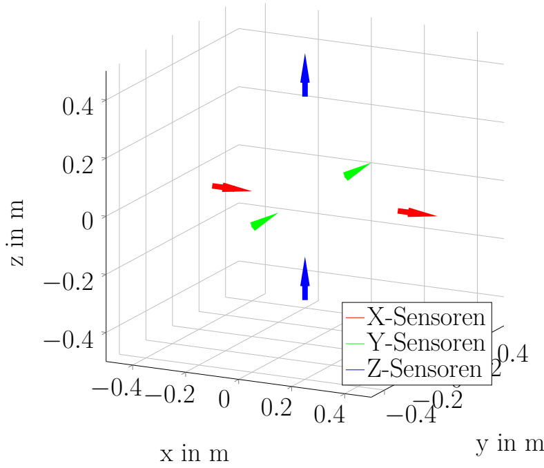
(a) Simulationssetup
