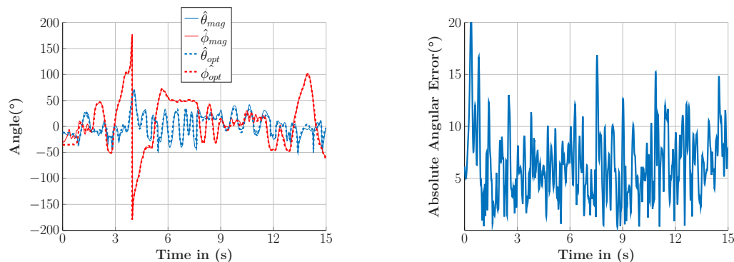
(a) Angle of movement for the second element (b) Magnitude of the angular error between optical and magnetic estimation
