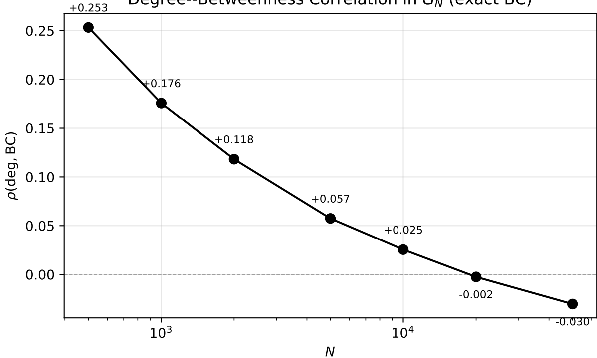
Degree--Betweenness Correlation in G_N (exact BC)
