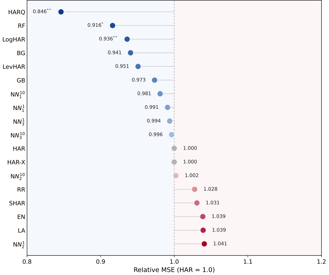
Figure 7: Cleveland Dot Plot of \mathcal{M}_{\text{HAR}} Results
