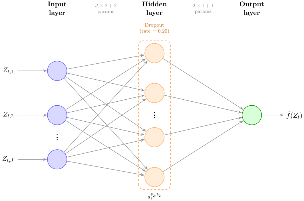
Figure 6: NN1 Feed-Forward Neural Network Architecture
