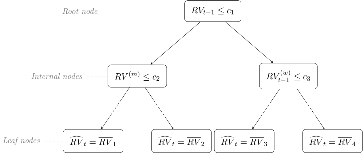
Figure 5: Illustration of a Regression Tree for Realized Variance
