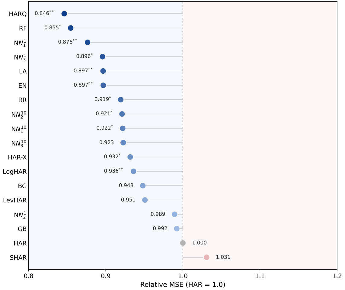
Figure 8: Cleveland Dot Plot of \mathcal{M}_{ALL} Results
