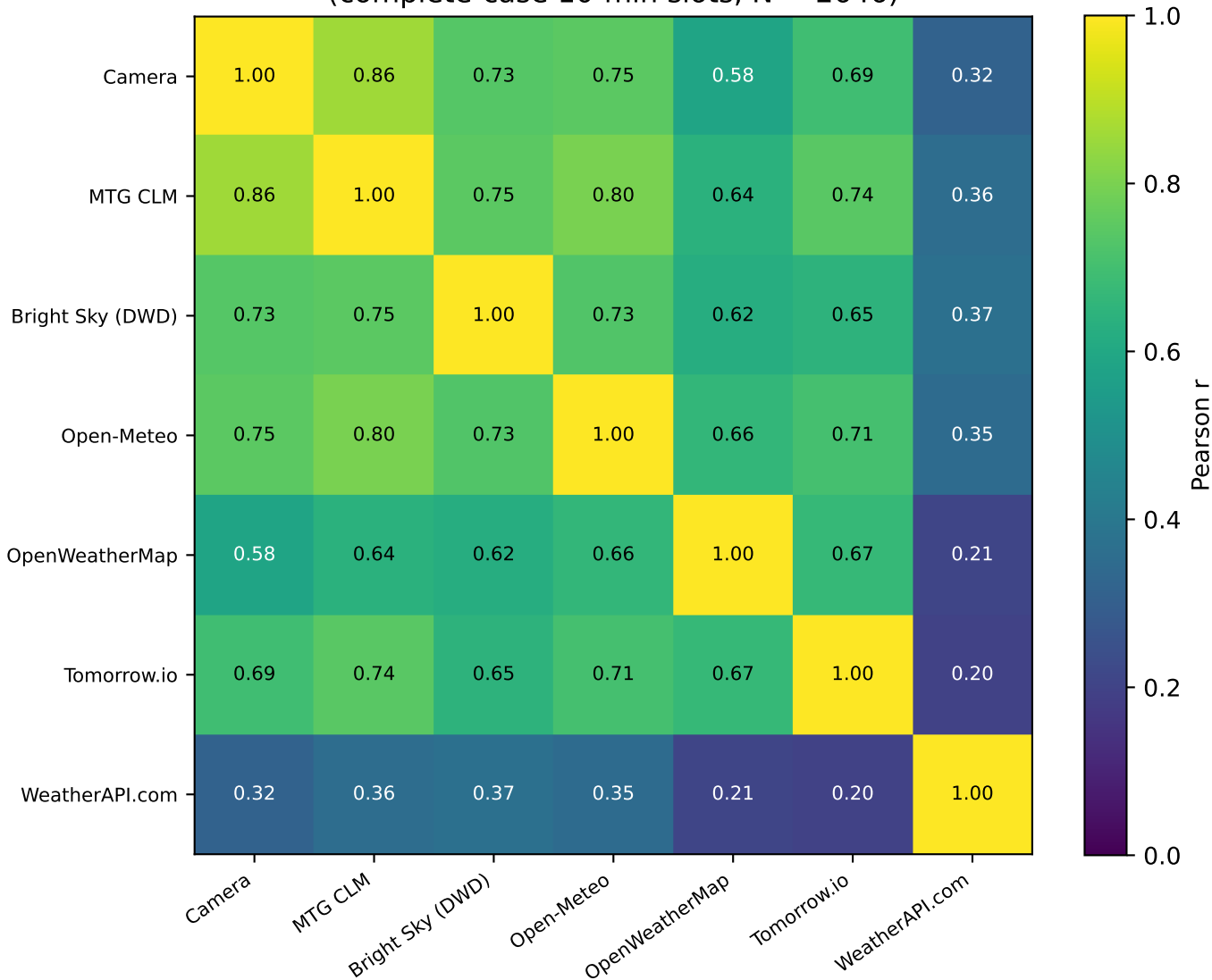
Pairwise correlation of cloud cover sources (complete-case 10-min slots, N = 2646)
