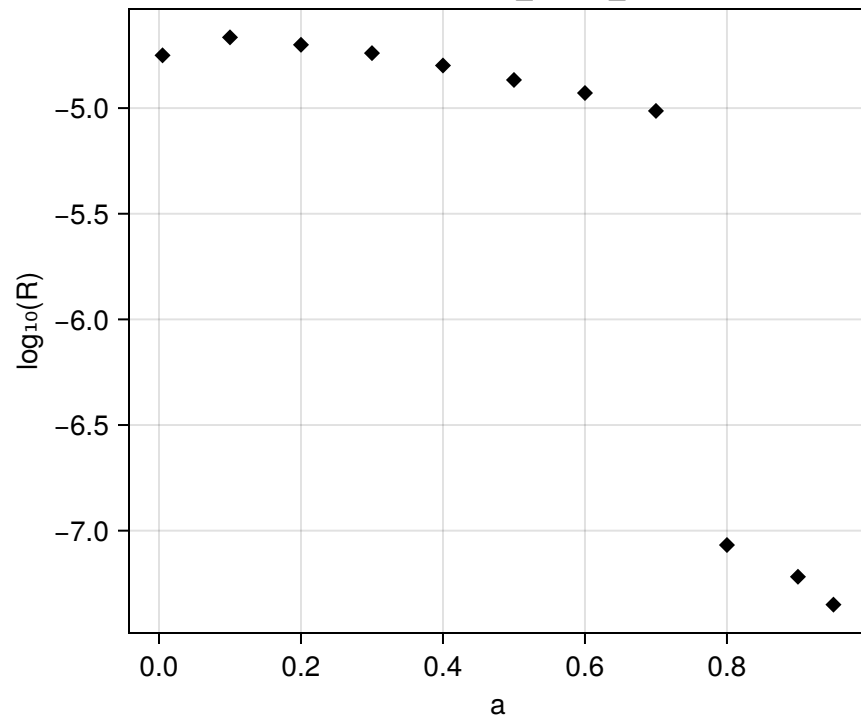
QEP residual \sigma_{\min}/\sigma_{\max}
