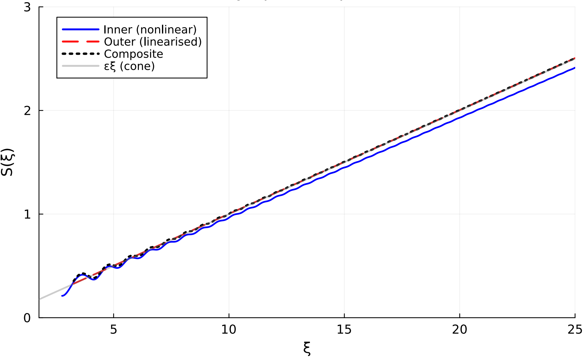
Matched asymptotic expansion ( \varepsilon=0.1 )
