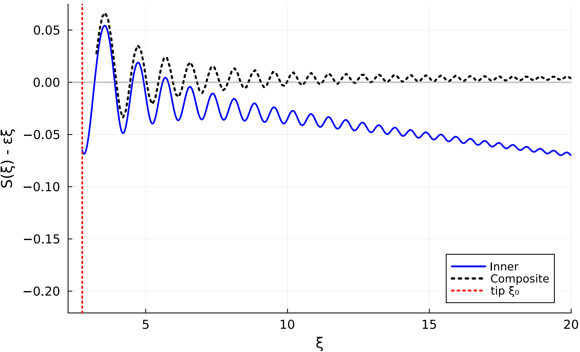
Blob + capillary waves ( \varepsilon=0.1 )
