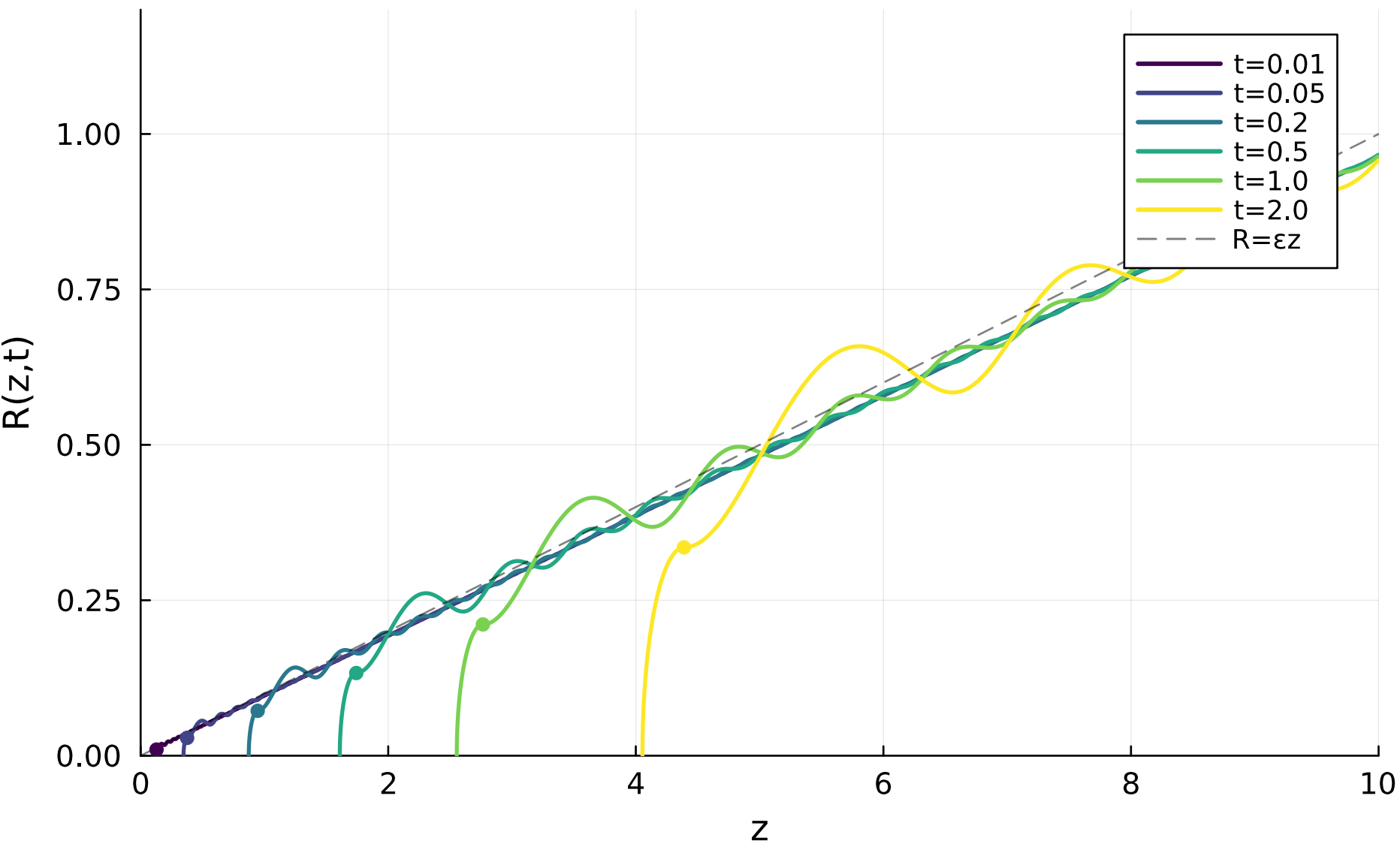
Cone tip recoil: profile at different times ( \varepsilon=0.1 )
