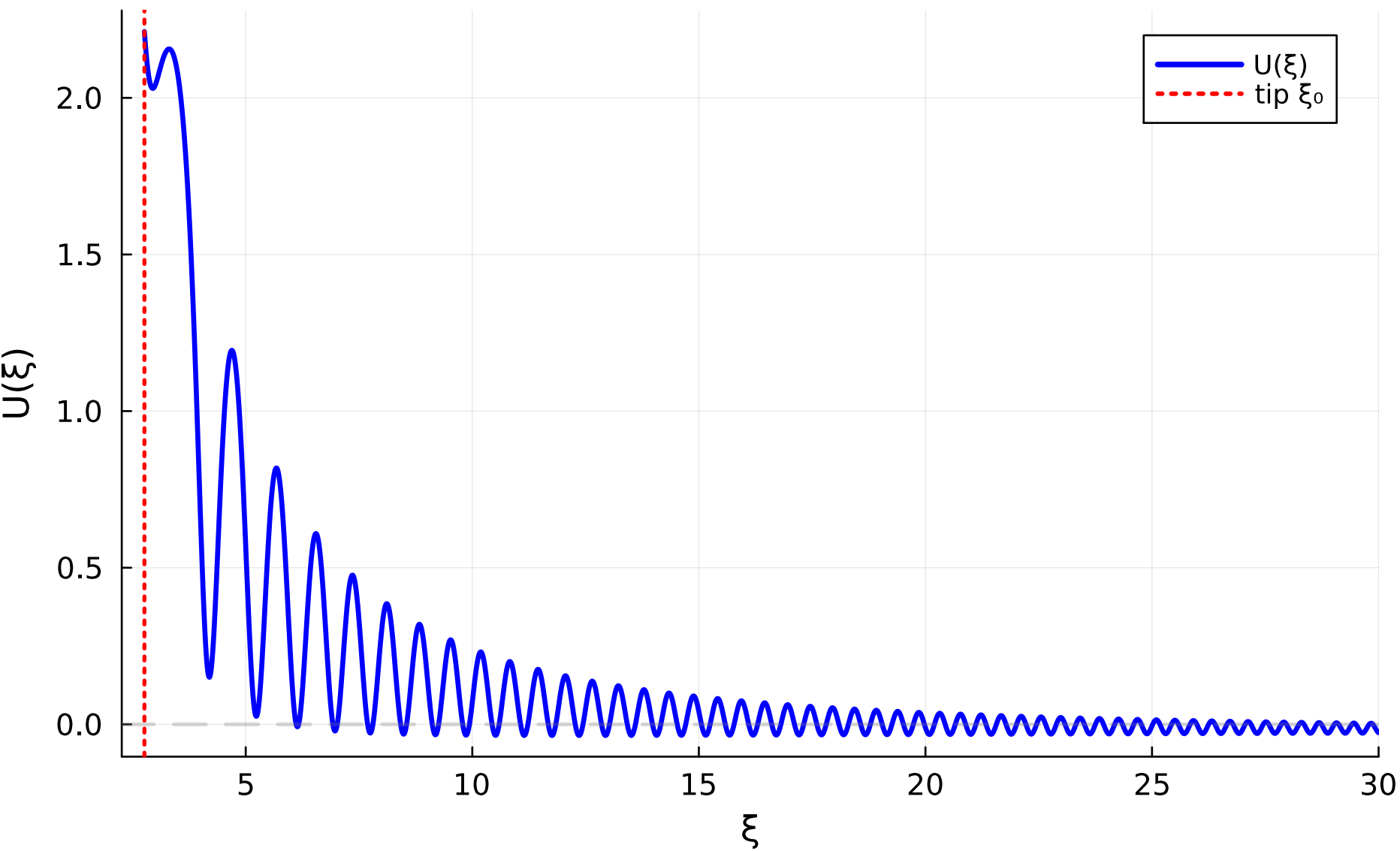
Similarity velocity ( \varepsilon=0.1 ): fluid pushed away from tip
