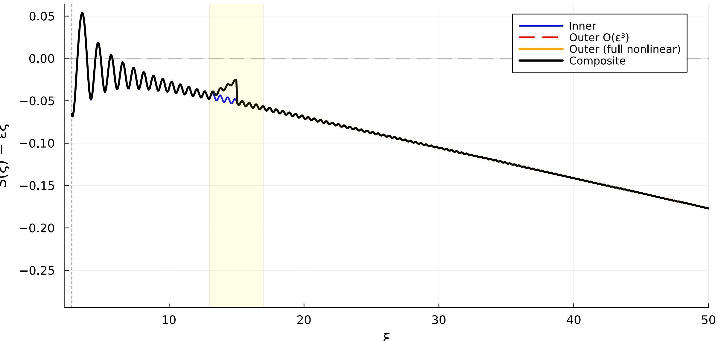
Linearised O(\varepsilon^3) vs full nonlinear outer ( \varepsilon=0.1 )
