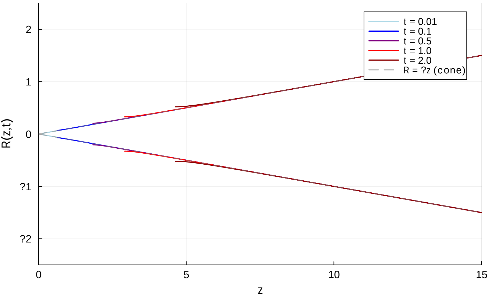
Recoiling cone: radius profile at different times
