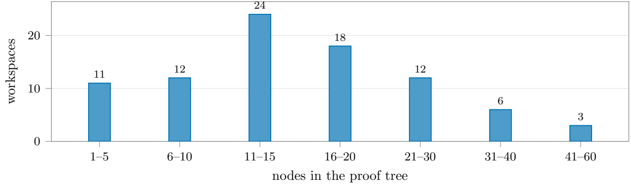
Figure 4: Size distribution of the 86 adversarial proof trees. The median tree has 14 nodes; the largest, lem-residual-upper , has 52.
