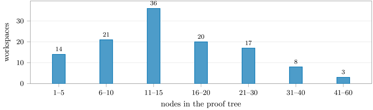
Figure 4: Size distribution of the 119 adversarial proof trees. The median tree has 14 nodes; the largest, lem-residual-upper , has 52.
