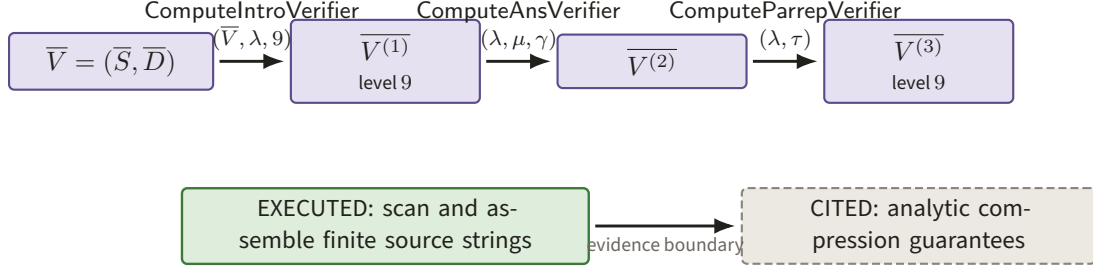
Figure 42. The compression program successively constructs \overline{V}^{(1)} , \overline{V}^{(2)} , \overline{V}^{(3)} by introspection, answer reduction, and repetition, with finite string assembly in green and analytic guarantees behind the dashed boundary. This separation matters because the compiler executes on descriptions even where soundness is supplied by cited theorems.
