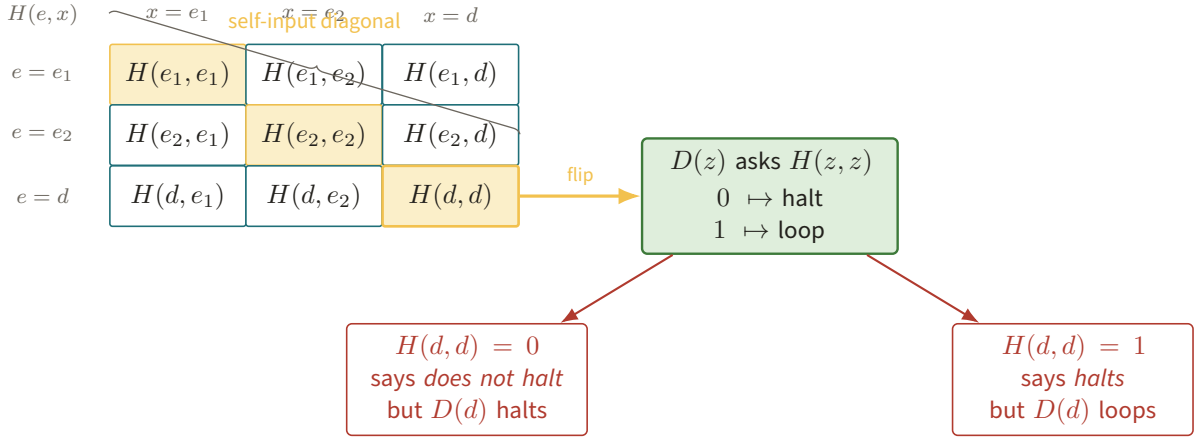
Figure 13. The amber diagonal specializes H(e, x) to self-inputs, and D reverses the highlighted value H(d, d) . Both possible bits terminate in a red contradiction, so no total table-filling decoder H can exist.
