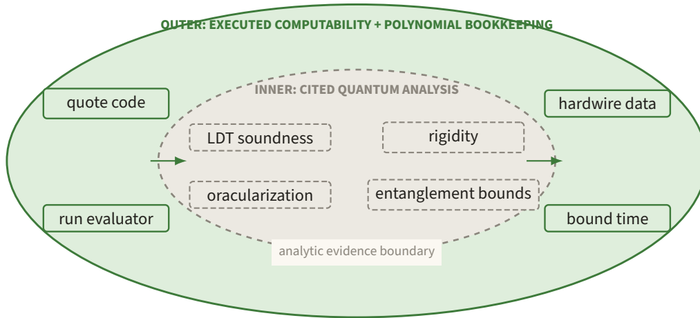
Figure 37. The green outer ring executes quotation, hardwiring, evaluation, and polynomial bookkeeping around a dashed slate core of LDT soundness, rigidity, oracularization, and entanglement bounds. Keeping this evidence boundary visible prevents source-level mechanization from being mistaken for a proof of the quantum analytic theorems.
