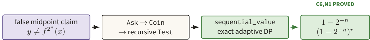
Figure 90. The Ask/Coin/Test recurrence is evaluated by an exact adaptive dynamic program. Its one-copy and sequential-AND values are the proved C6 and N1 formulas, not claims about quantum parallel repetition.
