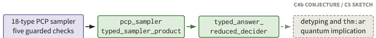
Figure 89. The 18-type sampler and guarded answer-reduced decider have constructed or finite-checked shapes. Detying and the quantum implication in thm:ar remain dashed at C4b CONJECTURE and C5 SKETCH.
