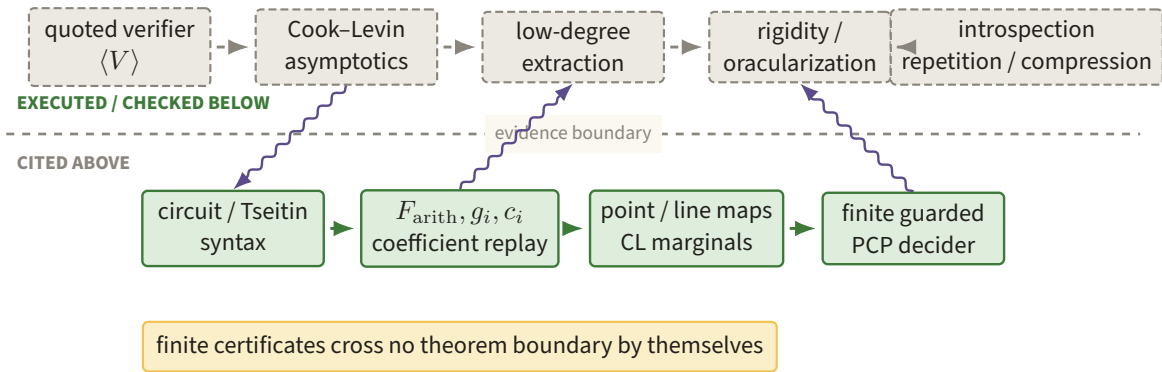
Figure 92. Green construction and replay stages sit below the boundary, while Cook–Levin asymptotics, low-degree extraction, rigidity, introspection, repetition, and compression remain dashed cited leaves above it. Violet crossings indicate interfaces, not a promotion of finite certificates into analytic theorems.
