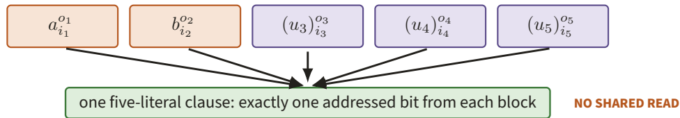
Figure 70. A decoupled clause reads exactly one addressed literal from each of a, b, u_3, u_4, u_5 , with the two answer blocks distinguished in rust. Independent low-degree answers can now supply the five locations without pretending to be three reads of one shared assignment.
