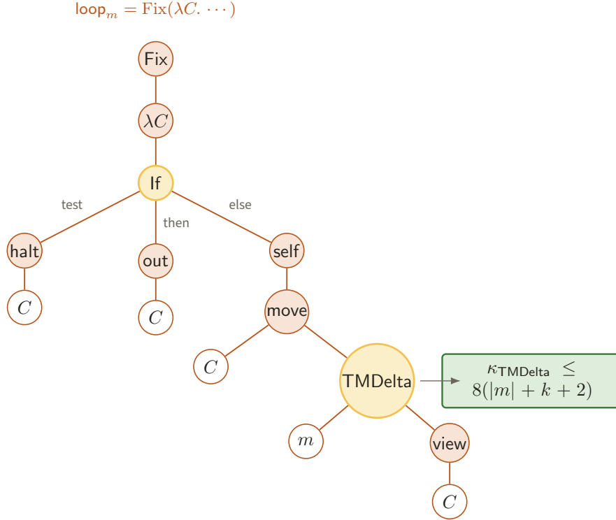
Figure 54. The tree for \text{loop}_m tests the current configuration, emits its output on halt, and otherwise feeds \text{move}(C, \text{TMDelta}(m, \text{view}(C))) through the self link. The amber table node isolates the only m -dependent per-iteration charge, bounded by 8(|m| + k + 2) .
