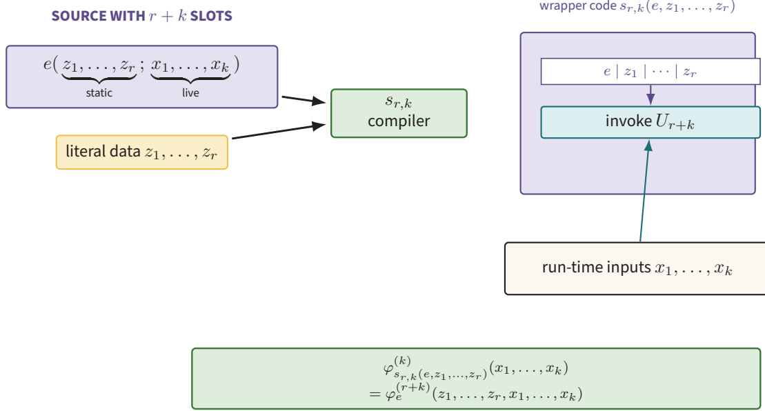
Figure 12. The s_{r,k} compiler moves e, z_1, \dots, z_r into a literal byte region while preserving x_1, \dots, x_k as run-time inputs. The resulting wrapper realizes parameter fixing by one finite source transformation followed by universal simulation.
