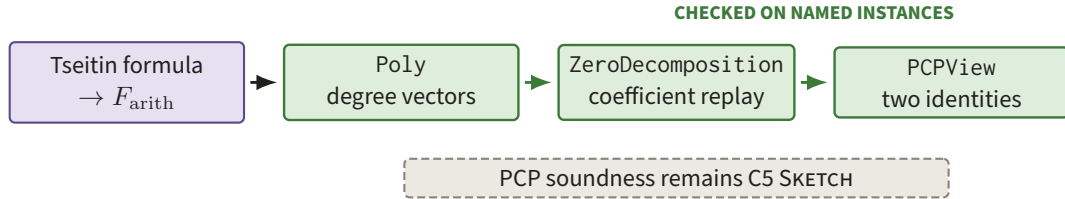
Figure 87. Tseitin syntax flows into sparse polynomials, exact zero-basis division, and the two local PCP identities. Green boxes are checked on named instances, while the separate dashed soundness leaf remains C5 SKETCH.
