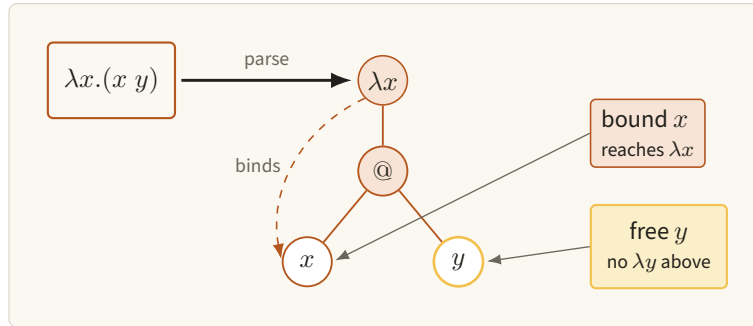
Figure 18. The tree for \lambda x.(x\ y) links the binder to its bound x while amber isolates the free y . Scope is structural, so consistent renaming changes labels without changing this graph.
