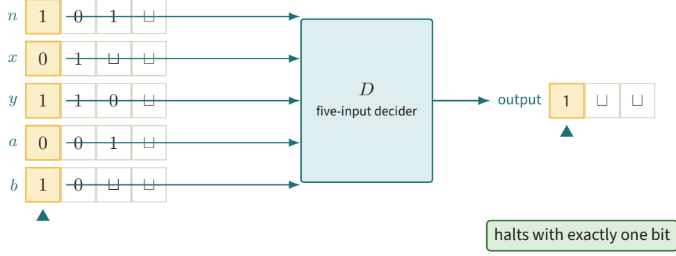
Figure 39. Five independent input tapes feed n, x, y, a, b to the decider, whose output tape must contain exactly one halting bit. Bounding the worst run at fixed n therefore also bounds how far any head can inspect the other four tapes.
