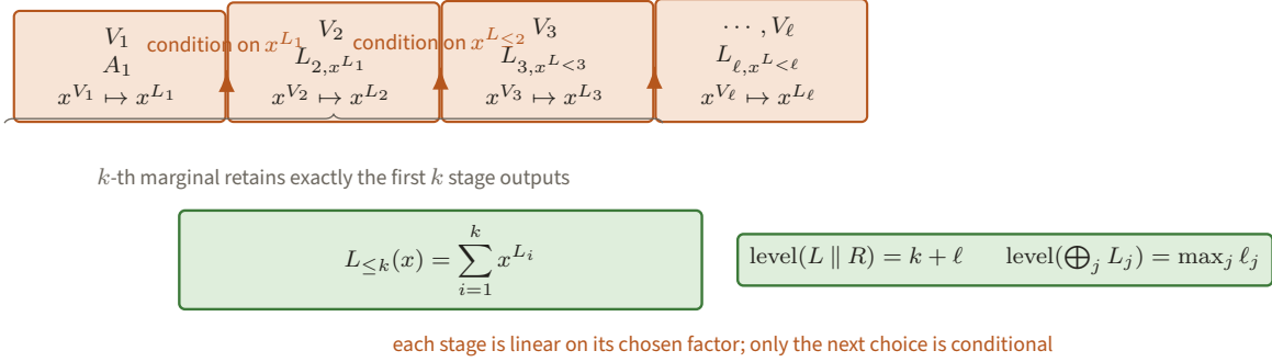
Figure 79. Each rust stage applies a linear map on one complementary register, while the labelled dependency lets earlier outputs select the next stage. Marginals sum prefixes of stage outputs, concatenation adds levels, and direct sum takes their maximum.
