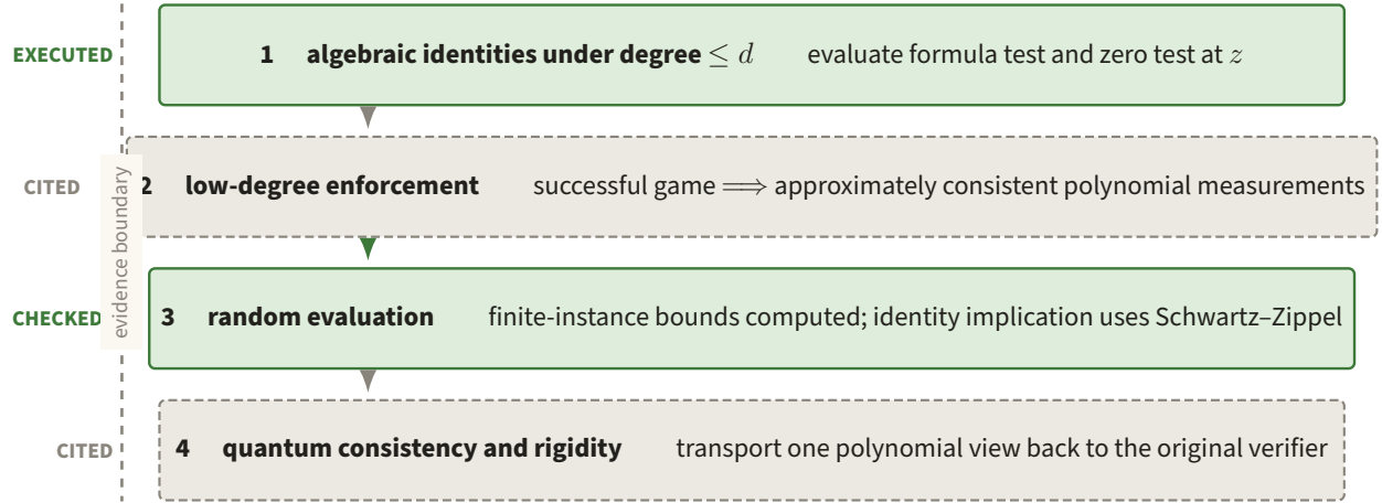
Figure 77. Green strata are computations or finite checks, while dashed slate strata are imported low-degree and quantum implications. The boundary prevents successful local evaluations from being mistaken for a proof of soundness against arbitrary strategies.
