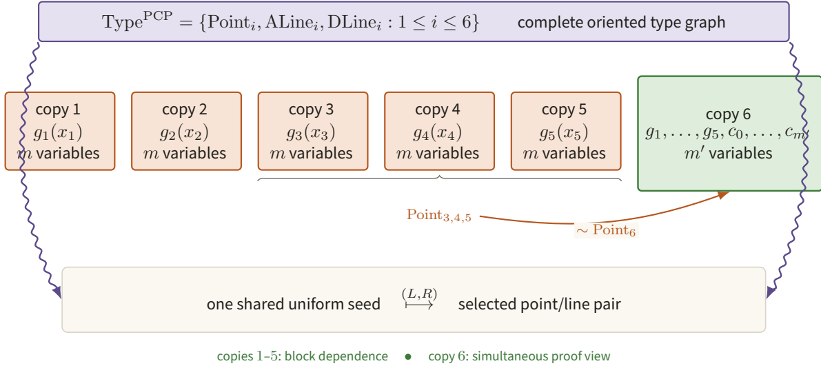
Figure 81. Copies one through five test the five block polynomials individually, while copy six tests the complete (g_1, \dots, g_5, c_0, \dots, c_{m'}) bundle in dimension m' . The 18 point/axis-line/diagonal-line types share one ambient seed and a complete oriented type graph.
