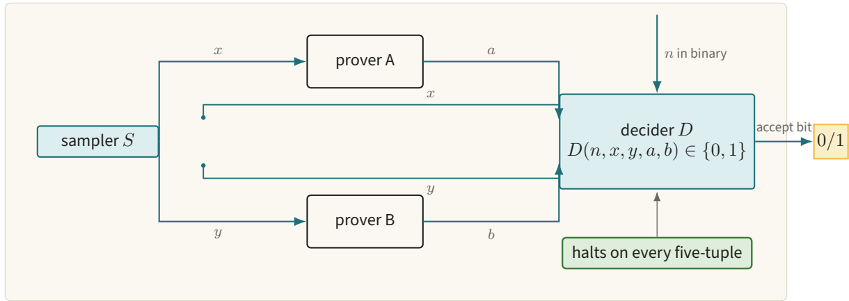
Figure 8. The sampler sends x, y to the two provers, while the total decider receives the copied questions together with n and returned answers a, b . This five-port interface is the normal form preserved by the later source transformations.
