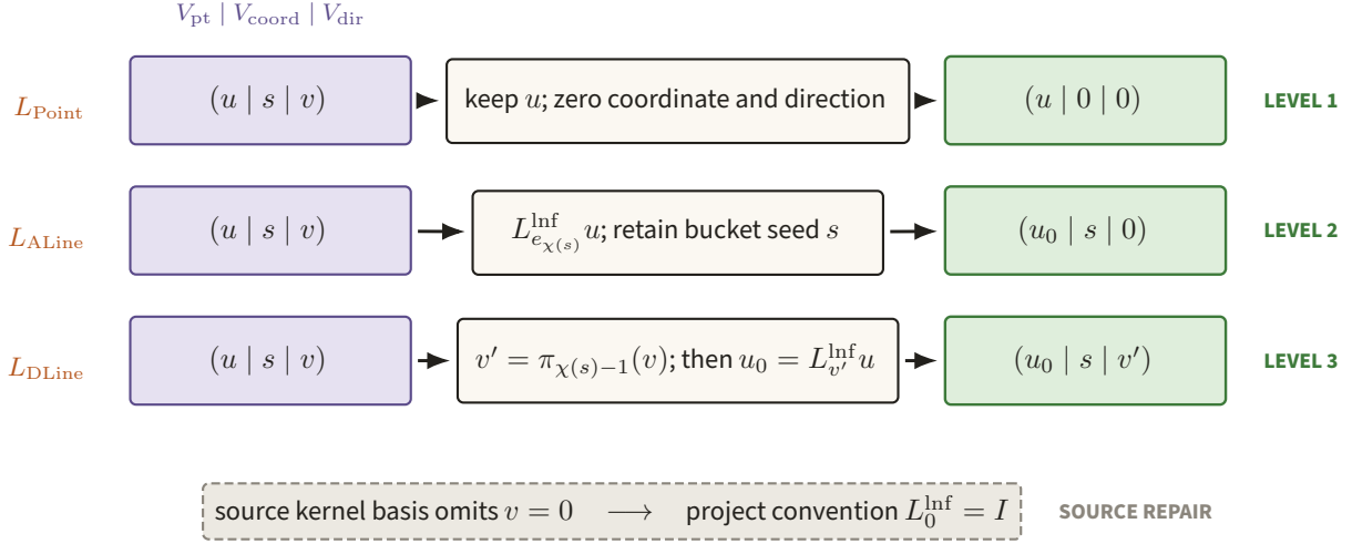
Figure 80. The point, axis-line, and diagonal-line maps act on the same V_{\text{pt}} \oplus V_{\text{coord}} \oplus V_{\text{dir}} seed but retain different register data. Their one-, two-, and three-level factorizations make the sampled geometry CL, with L_0^{\text{lnf}} = I visibly marked as a source repair.
