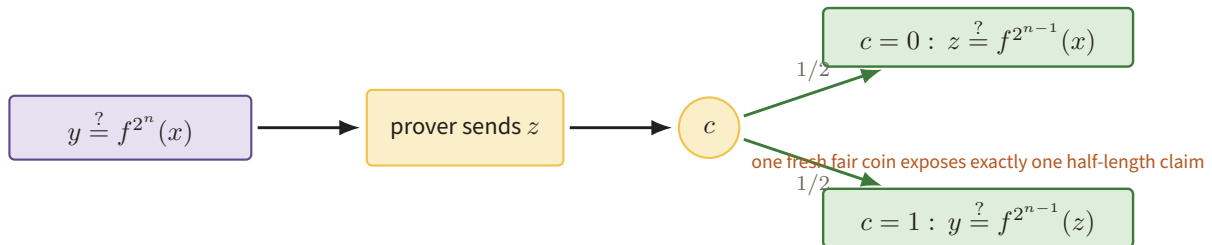
Figure 94. After the prover supplies z , one fresh fair coin selects the left or right half-length orbit claim. This single branching move yields the exact false-claim recurrence behind p_n = 1 - 2^{-n} .
