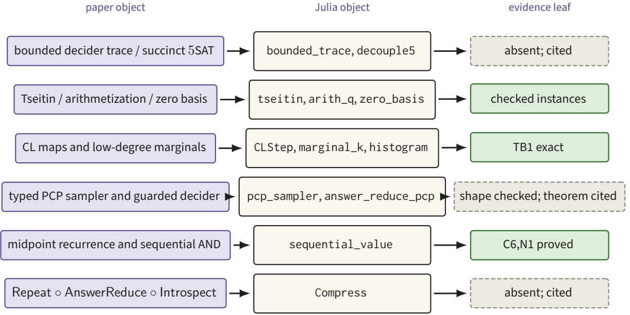
Figure 85. Each row aligns a paper object with its current Julia representation and the narrowest evidence leaf actually available. Green instance checks occupy the middle rungs, while missing front-end and compression implementations remain visibly cited.
