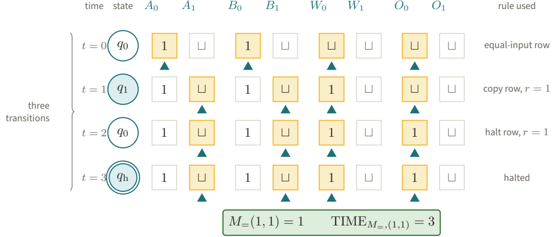
Figure 7. Four time rows track the A, B, W, O tapes of M_= , with amber cells and triangles marking every scanned symbol and head. The rule labels expose why equal inputs produce output one and reach q_h after exactly three transitions.
