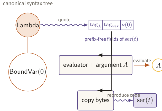
Figure 32. The identity tree quotes through a violet wavy arrow to canonical prefix-free fields, which an evaluator maps with A to A while a copier returns the fields themselves. Quotation reifies finite syntax without confusing code with the value obtained by running it.
