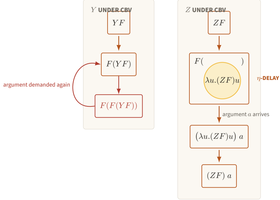
Figure 30. Under call-by-value, YF repeatedly demands its recursive argument, while ZF parks the same demand beneath the amber abstraction \lambda u . The delayed branch unfolds only when a concrete argument arrives, making Z the appropriate fixed point for the project evaluator.
