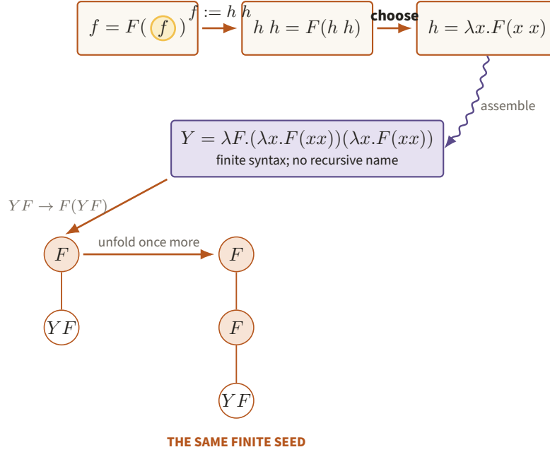
Figure 28. The fixed-point equation is solved by self-application, yielding finite Y syntax whose reduction grows the tree F(YF), F(F(YF)), \dots . Recursion is produced by running the seed rather than by storing an infinite or recursively named term.
