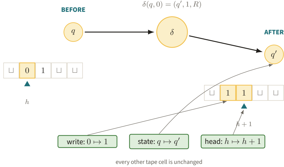
Figure 4. The amber transition rewrites the scanned zero, changes q to q' , and advances the head from h to h + 1 . Exposing exactly these three local changes is what later permits a computation history to be checked by bounded windows.
