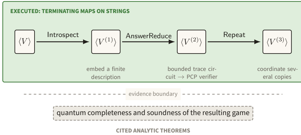
Figure 36. The green description pipeline embeds code, builds the bounded-trace PCP verifier, and coordinates copies before stopping at a dashed evidence boundary. Executing these finite transformations constructs the game but does not establish the cited quantum completeness and soundness theorem.
