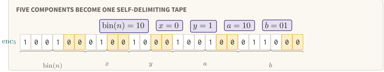
Figure 38. Dual rail turns each data bit into a two-cell codeword and marks every component boundary by the amber 00 delimiter. The same self-delimiting tape is consumed on both sides of the machine–term translation.
