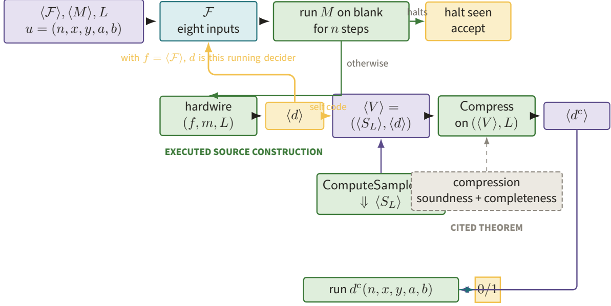
Figure 17. The eight-input machine first accepts a witnessed n -step halt; otherwise it hardwires (f, m, L) , feeds the resulting self-code d into (S_L, d) , compresses, and runs the returned decider. Green boxes are executed source operations while the dashed slate box is the cited game-theoretic guarantee (after fig:halt_f).
