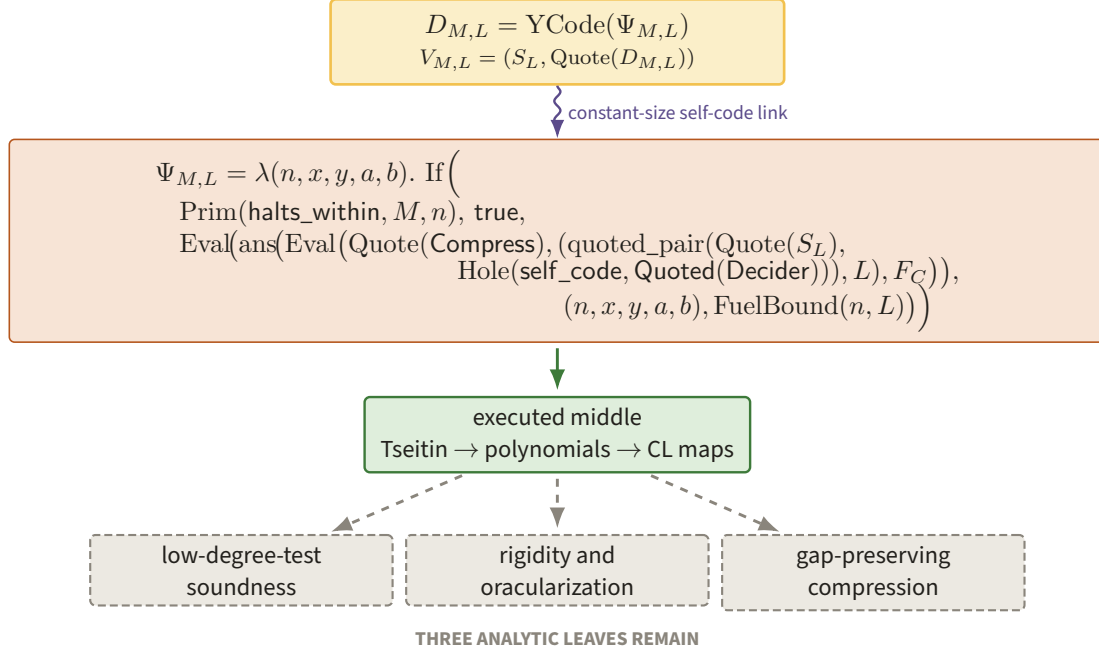
Figure 95. The actual term \Psi_{M,L} places its self-code hole inside the quoted call to Compress , and the amber fixed point D_{M,L} = \text{YCode}(\Psi_{M,L}) closes that hole with constant overhead. The executable algebraic middle does not discharge the three dashed leaves: low-degree soundness, rigidity/oracularization, and gap-preserving compression.
