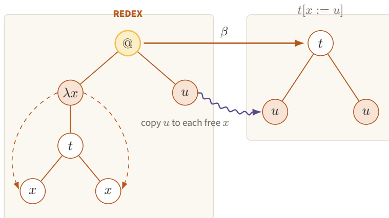
Figure 19. The amber application is cut away and the argument subtree u is spliced into every free x -leaf of t . This concrete operation is the term-level model for later code specialization.
