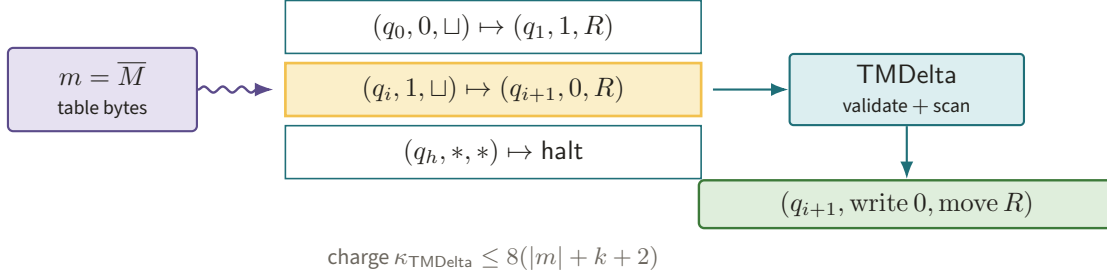
Figure 53. The TMDelta primitive validates and scans the bytes of m until the current state-symbol tuple selects one row, then returns the next state, write symbols, and motions. Keeping the table as data explains both the single-copy description size and charge 8(|m| + k + 2) .
