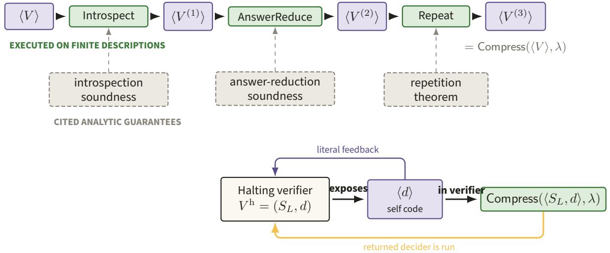
Figure 1. Green stages are finite source transformations, while dashed slate boxes mark the analytic guarantees they invoke and the amber return path closes the self-code loop. The split keeps executable description manipulation visibly separate from cited soundness in the compression argument (after fig:compress).
