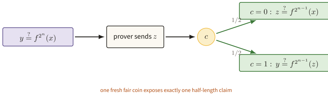
Figure 109. After the prover supplies z , one fresh fair coin selects the left or right half-length orbit claim. This single branching move yields the exact false-claim recurrence behind p_n = 1 - 2^{-n} .
