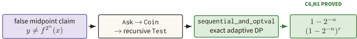
Figure 103. The Ask/Coin/Test recurrence is evaluated by an exact adaptive dynamic program. Its one-copy and sequential-AND values are the proved C6 and N1 formulas, not claims about quantum parallel repetition.
