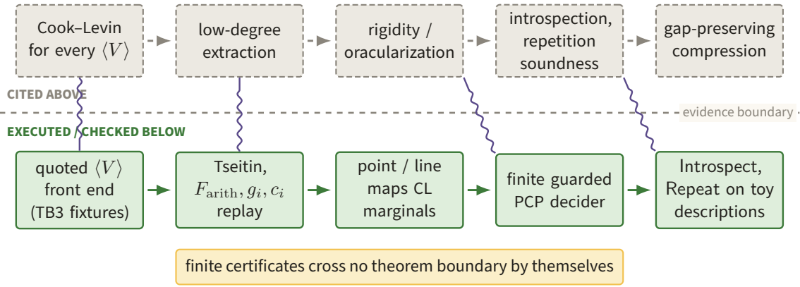
Figure 106. Green construction and replay stages, now including the TB3 front end and the built TB5–TB6 transformations on toy descriptions, sit below the boundary, while Cook-Levin for every description, low-degree extraction, rigidity, introspection and repetition soundness, and gap-preserving compression remain dashed cited leaves above it. Violet crossings indicate interfaces, not a promotion of finite certificates into analytic theorems.
