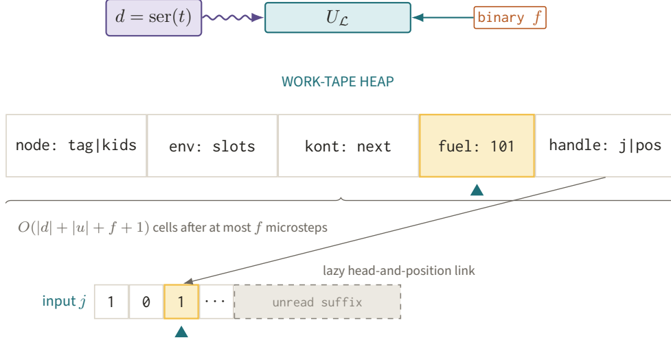
Figure 62. The work tape of U_{\mathcal{L}} stores syntax nodes, environments, continuations, binary fuel, and lazy input handles as finite records, with the active fuel record highlighted. Because a handle reaches only the visited prefix, an f -unit run is independent of every dashed unread suffix.
