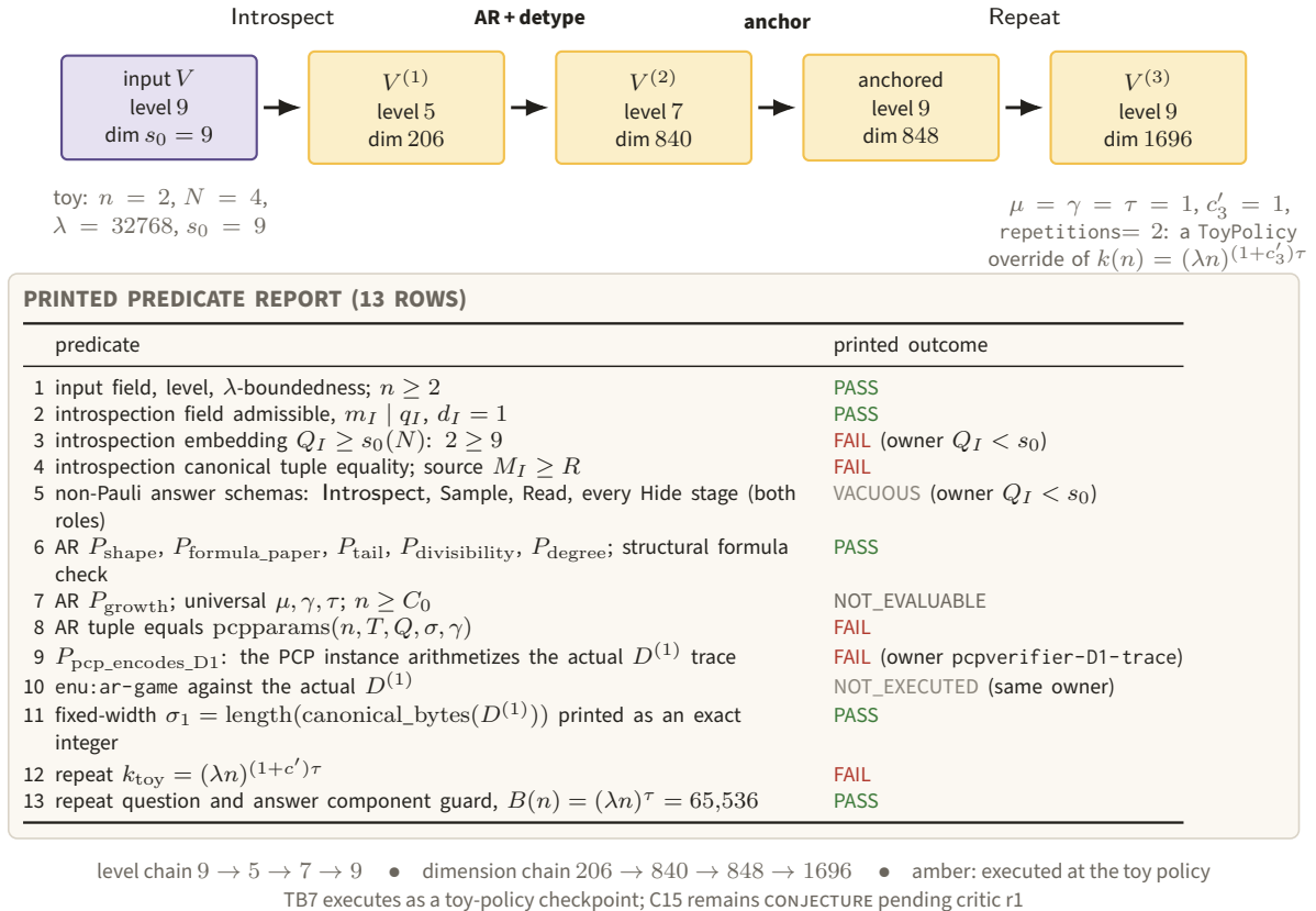
Figure 105. The TB7 toy-policy checkpoint at n = 2 , \lambda = 32768 , s_0 = 9 : the constructed level and dimension chains and all thirteen printed predicate outcomes, with every FAIL, VACUOUS, NOT_EVALUABLE and NOT_EXECUTED row kept beside the chain. Printing the failures beside the chain is what keeps an executed construction from reading as a discharged theorem; C15 remains CONJECTURE pending critic r1.
