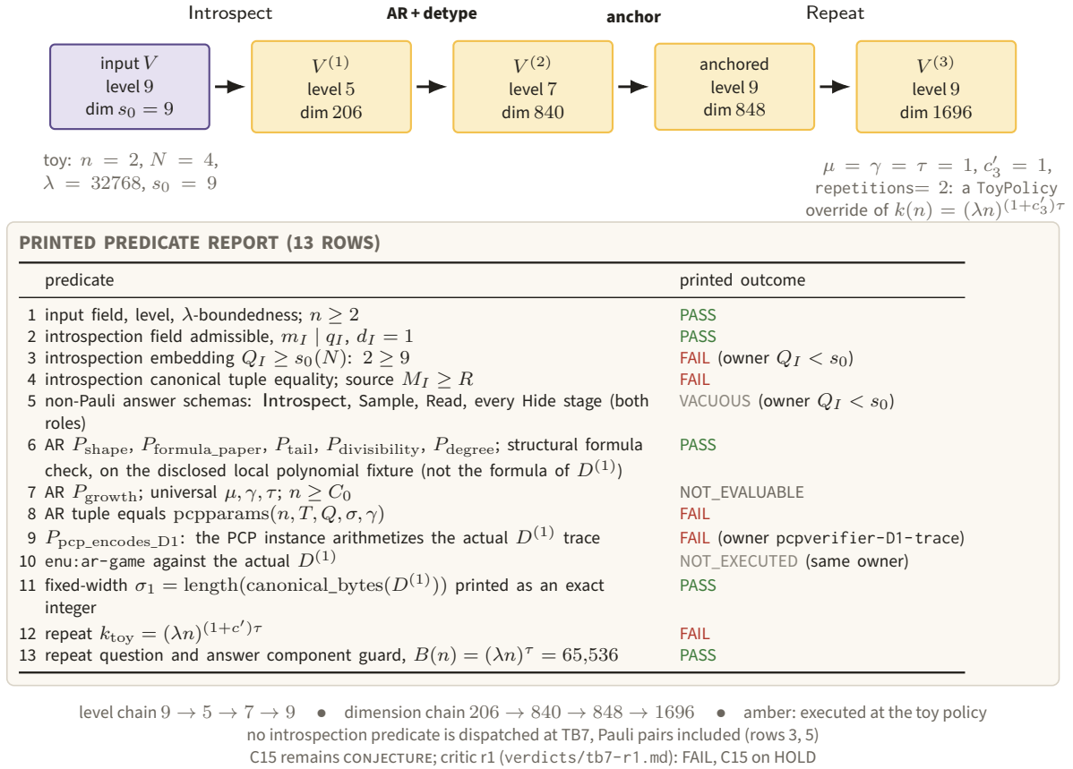
Figure 106. The TB7 toy-policy checkpoint at n = 2 , \lambda = 32768 , s_0 = 9 : the constructed level and dimension chains and all thirteen printed predicate outcomes, with every FAIL, VACUOUS, NOT_EVALUABLE and NOT_EXECUTED row kept beside the chain. Printing the failures beside the chain is what keeps an executed construction from reading as a discharged theorem. Row 6’s PASS is on the disclosed local polynomial fixture, not on the formula of D^{(1)} . C15 remains CONJECTURE; critic r1 returned FAIL/HOLD.
