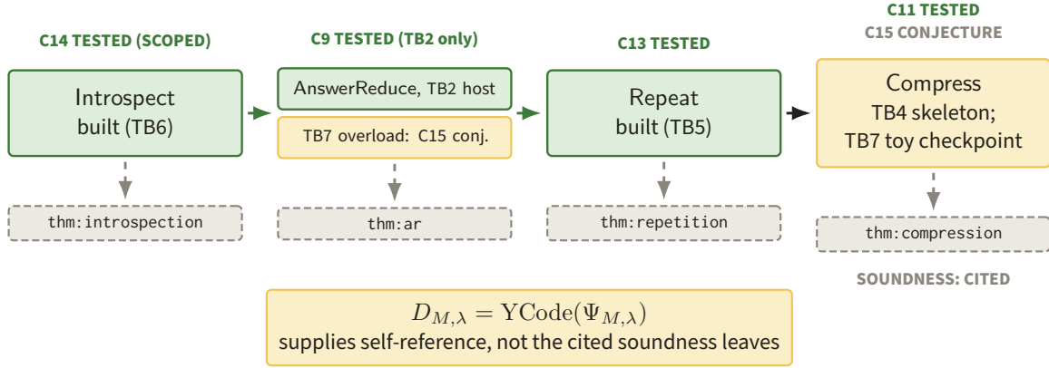
Figure 105. Introspection, answer reduction, and repetition are built transformations that compose, in the fig:compress order, into the Compress row (C11 for the TB4 skeleton; TB7 a toy-policy checkpoint with C15 CONJECTURE), while their soundness leaves remain dashed and cited. Answer reduction is split in two: C9 TESTED covers only the TB2 host-object construction on its proof/formula fixture, and the TB7 description overload belongs to C15, whose actual- D^{(1)} game is not executed. The amber fixed point supplies self-reference only; it does not discharge those analytic contracts.
