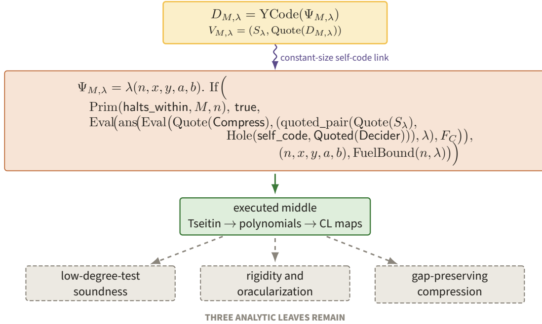
Figure 108. The actual term \Psi_{M,\lambda} places its self-code hole inside the quoted call to Compress , and the amber fixed point D_{M,\lambda} = \text{YCode}(\Psi_{M,\lambda}) closes that hole with constant overhead. The executable algebraic middle does not discharge the three dashed leaves: low-degree soundness, rigidity/oracularization, and gap-preserving compression.
