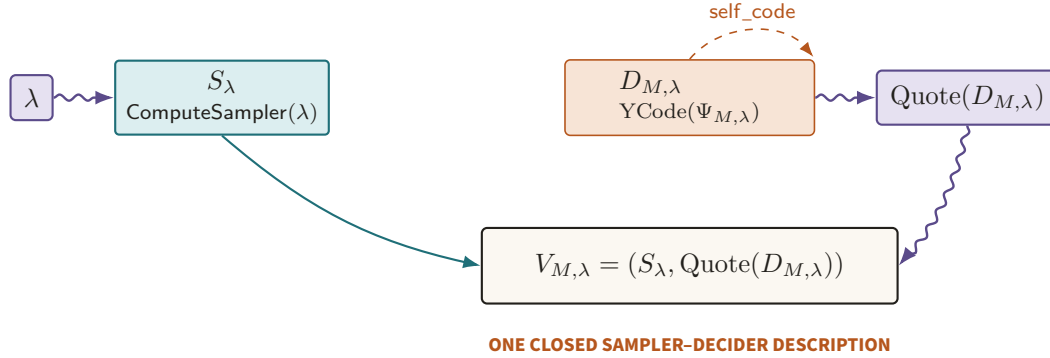
Figure 70. The literal bound \lambda produces S_\lambda , while \text{YCode}(\Psi_{M,\lambda}) closes its sole self-code socket before quotation places D_{M,\lambda} beside that sampler. The resulting V_{M,\lambda} is one finite normal-form verifier description, not an oracle for either component.
