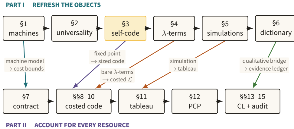
Figure 3. The upper path introduces machines, self-description, and lambda simulation before the lower path assigns sizes, costs, tableaux, and evidence grades. The vertical arrows name which qualitative refresher each resource-accounted construction upgrades; §2’s universal machine is used throughout rather than upgraded at one place, and §12’s PCP algebra is new material with no Part I counterpart.
