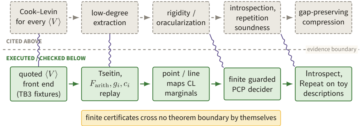
Figure 107. Green construction and replay stages, now including the TB3 front end and the built TB5–TB6 transformations on toy descriptions, sit below the boundary, while Cook–Levin for every description, low-degree extraction, rigidity, introspection and repetition soundness, and gap-preserving compression remain dashed cited leaves above it. Violet crossings indicate interfaces, not a promotion of finite certificates into analytic theorems.
