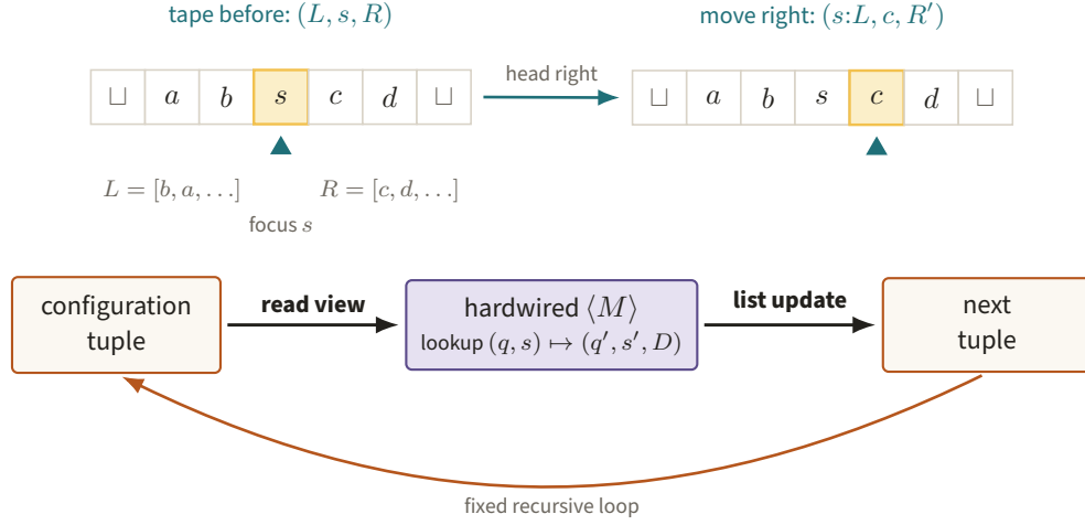
Figure 33. A right move rethreads the focused tape cell s from the zipper’s right edge onto L and focuses c , while a fixed loop consults the one hardwired copy of \langle M \rangle . Local list updates simulate machine steps without duplicating the transition table.
