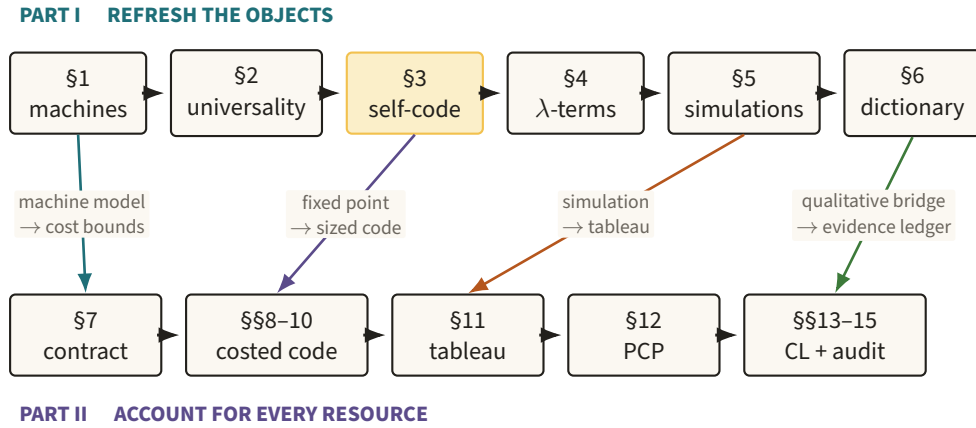
Figure 2. The upper path introduces machines, self-description, and lambda simulation before the lower path assigns sizes, costs, tableaux, and evidence grades. The vertical arrows identify exactly which qualitative refresher each resource-accounted construction upgrades.
