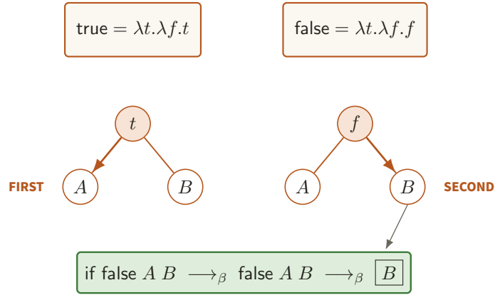
Figure 23. true and false route the same two continuations to opposite outputs, with if false A \ B selecting B . A Church bit is therefore its elimination behavior, exactly the interface later implemented by a primitive conditional.
