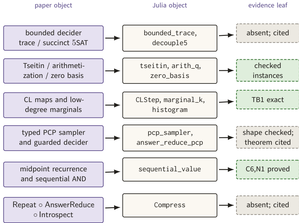
Figure 90. Each row aligns a paper object with its current Julia representation and the narrowest evidence leaf actually available. Green instance checks occupy the middle rungs, while missing front-end and compression implementations remain visibly cited.
