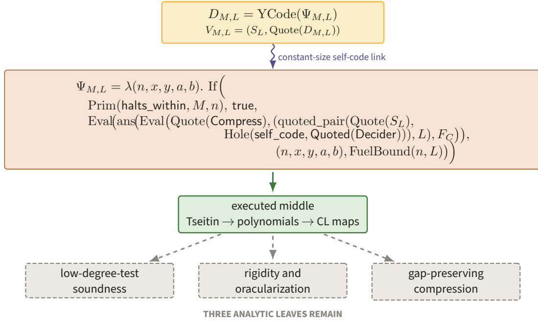
Figure 100. The actual term \Psi_{M,L} places its self-code hole inside the quoted call to Compress , and the amber fixed point D_{M,L} = \text{YCode}(\Psi_{M,L}) closes that hole with constant overhead. The executable algebraic middle does not discharge the three dashed leaves: low-degree soundness, rigidity/oracularization, and gap-preserving compression.
