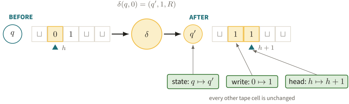
Figure 4. The amber transition rewrites the scanned zero, changes q to q' , and advances the head from h to h + 1 . Exposing exactly these three local changes is what later permits a computation history to be checked by bounded windows.
