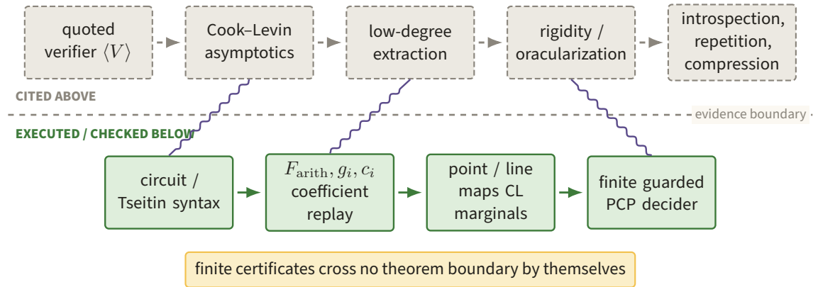
Figure 97. Green construction and replay stages sit below the boundary, while Cook–Levin asymptotics, low-degree extraction, rigidity, introspection, repetition, and compression remain dashed cited leaves above it. Violet crossings indicate interfaces, not a promotion of finite certificates into analytic theorems.
