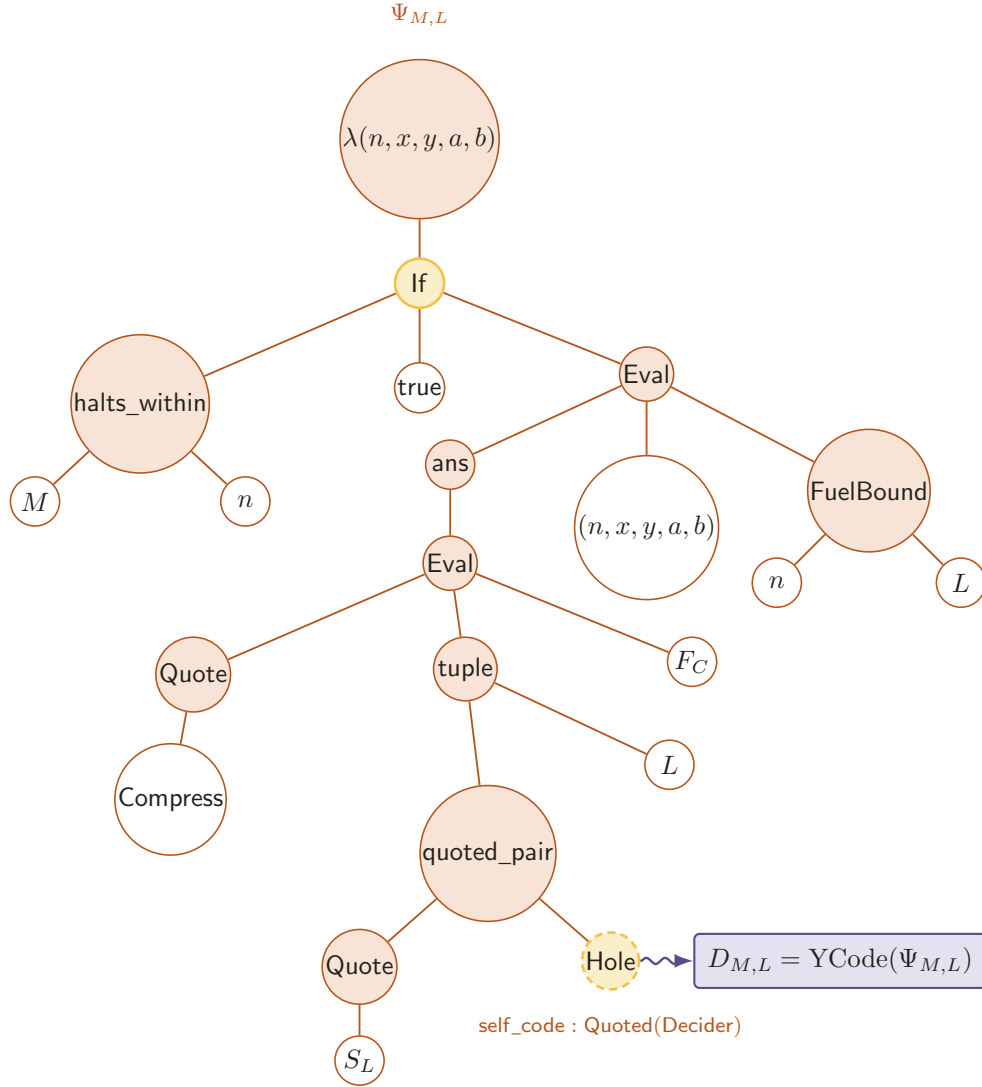
Figure 64. The real term \Psi_{M,L} first tests \text{halts\_within}(M, n) ; on failure it evaluates quoted Compress on (\text{quoted\_pair}(\text{Quote}(S_L), \text{Hole}(\text{self\_code})), L) , selects the answer decider, and evaluates it on (n, x, y, a, b) . The lone amber hole is exactly the source position closed by D_{M,L} = \text{YCode}(\Psi_{M,L}) .
