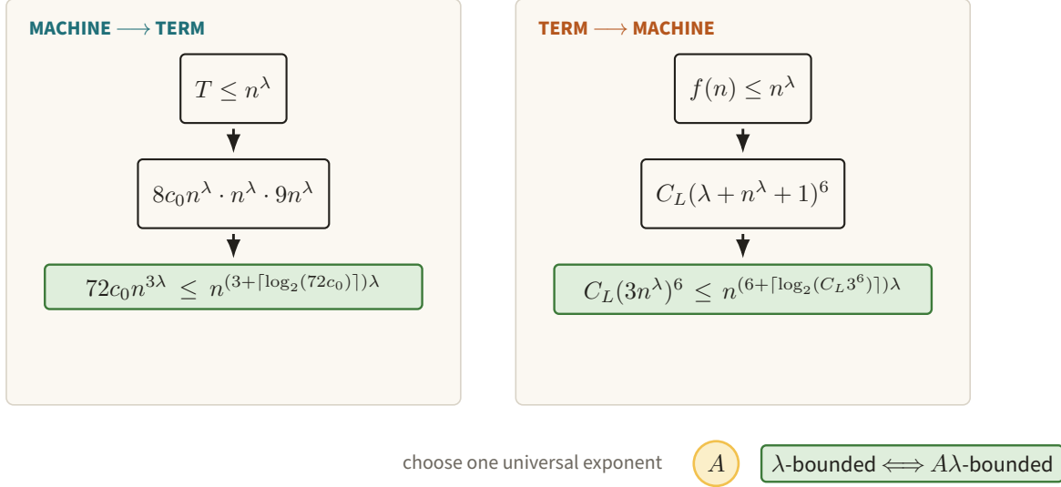
Figure 58. The machine-to-term direction contributes exponent 3 + \lceil \log_2(72c_0) \rceil , while the term-to-machine direction contributes 6 + \lceil \log_2(C_L 3^6) \rceil . Choosing one universal A above both calculations preserves the bounded verifier class in either language.
