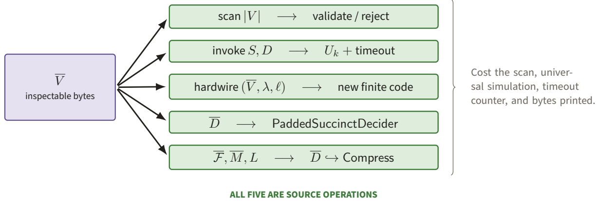
Figure 43. Every green branch starts from the actual bytes of \bar{V} : scan, universal invocation, hardwiring, Cook–Levin compilation, and the self-description fed to Compress. The bridge is intensional only if all five source operations remain finite and resource-accounted.
