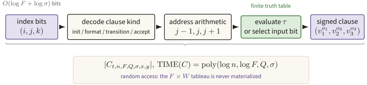
Figure 68. An O(\log F + \log \sigma) -bit index is decoded into one real initialization, format, transition, or acceptance clause. Random access keeps the description polynomial in \log F even though the underlying tableau has F time rows.
