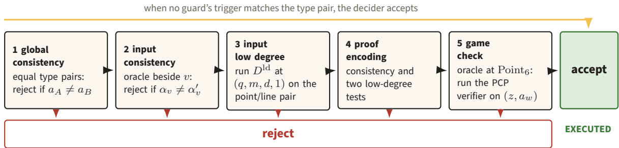
Figure 86. Acceptance flows left to right through five guards and every guard drops out downwards to the same rejection, so a type pair whose trigger never matches follows the amber path straight to acceptance. All five guards are finite executed code in the prototype, with proof encoding running its consistency test and low-degree tests at (q, m, d, 1) and (q, m', d, m' + 6) ; only the soundness theorem quantifying over them stays cited (after fig:decider-pcp ).
