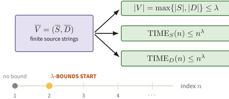
Figure 41. A single bound \lambda caps both source descriptions and both worst-case running times, with the time ruler beginning at n = 2 . This common scale is what can later be rescaled uniformly to A\lambda .
