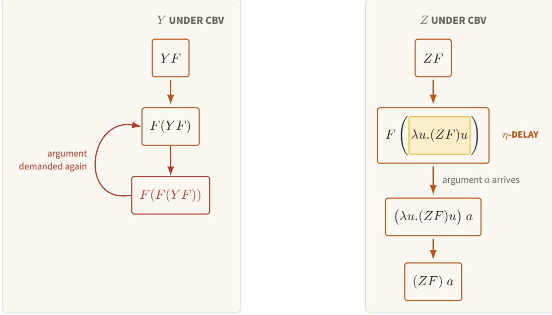
Figure 30. Under call-by-value, YF repeatedly demands its recursive argument, while ZF parks the same demand beneath the amber abstraction \lambda u. . The delayed branch unfolds only when a concrete argument arrives, making Z the appropriate fixed point for the project evaluator.
