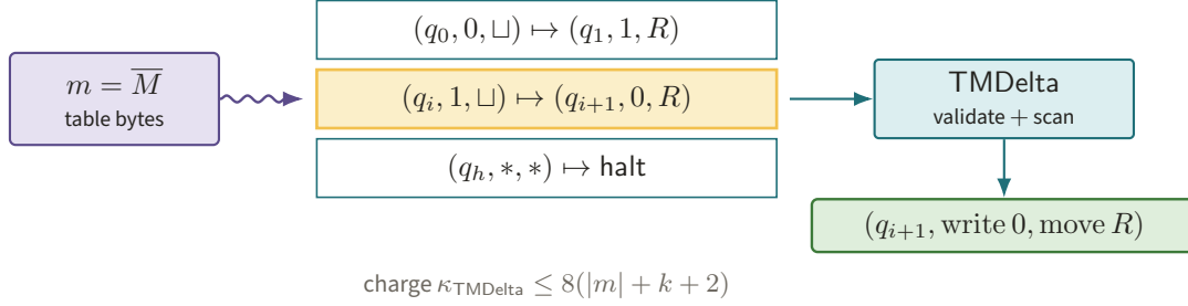
Figure 53. The TMDelta primitive validates and scans the bytes of m until the current state-symbol tuple selects one row, then returns the next state, write symbols, and motions. Keeping the table as data explains both the single-copy description size and charge 8(|m| + k + 2) .
