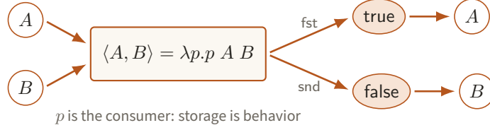
Figure 24. The Church pair stores A and B by passing both to a consumer p , while \text{true} and \text{false} project opposite components. Primitive tuples later preserve this interface while giving projection an explicit small cost.
