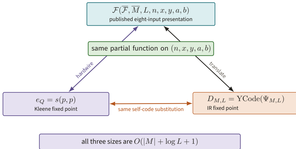
Figure 65. The published \mathcal{F}(\overline{\mathcal{F}}, \overline{M}, L, \dots) , Kleene's e_Q = s(p, p) , and D_{M,L} = \text{YCode}(\Psi_{M,L}) are three finite descriptions of the same partial function (after fig:halt_f ). Every edge preserves the self-code substitution and keeps size O(|M| + \log L + 1) .
