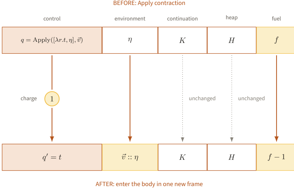
Figure 47. One Apply contraction replaces control by the body, pushes \vec{v} onto the environment, and changes fuel from f to f - 1 , leaving K and H untouched. Exposing all five registers makes the resource charge part of the operational state rather than an external annotation.
