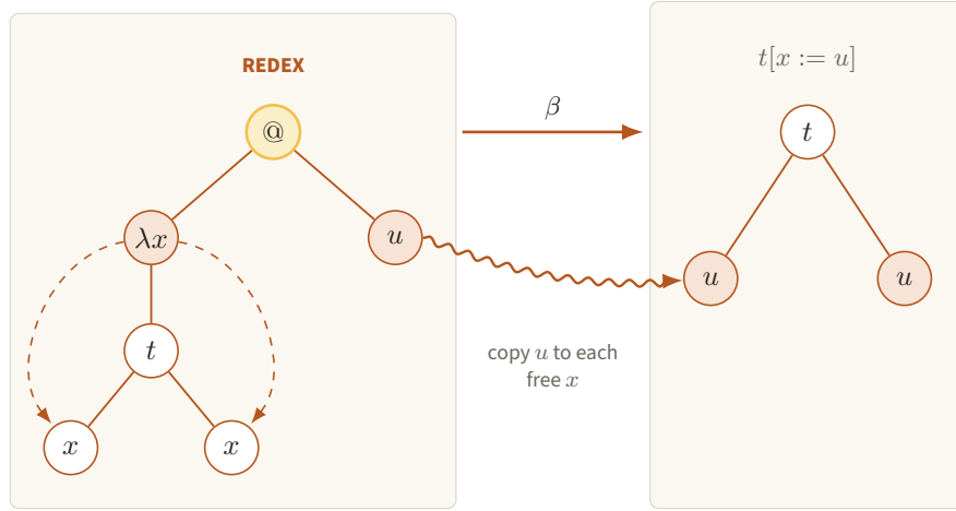
Figure 19. The amber application is cut away and the argument subtree u is spliced into every free x -leaf of t . This concrete operation is the term-level model for later code specialization.
