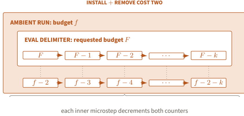
Figure 48. The Eval delimiter nests an F -unit budget inside ambient fuel f , charging two units for installation and removal and one from both counters per inner microstep. Exhausting either ledger therefore ends the same finite outer computation.
