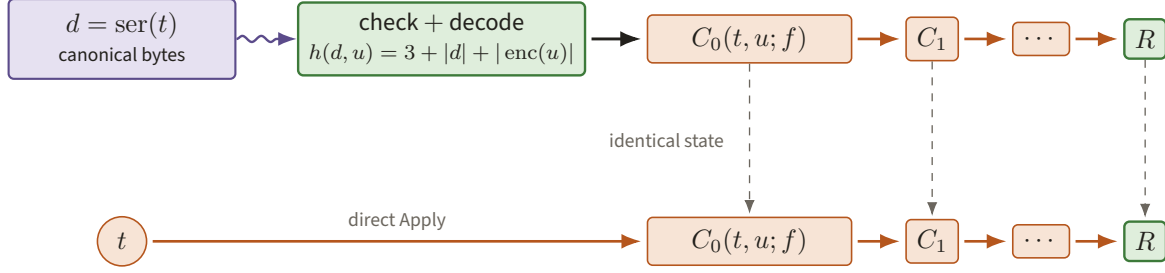
Figure 51. Quoted execution spends h(d, u) = 3 + |d| + |\text{enc}(u)| to decode canonical bytes and then lands on the direct run's exact initial CEK state. From that meeting point determinism forces both trajectories to return the same result.
