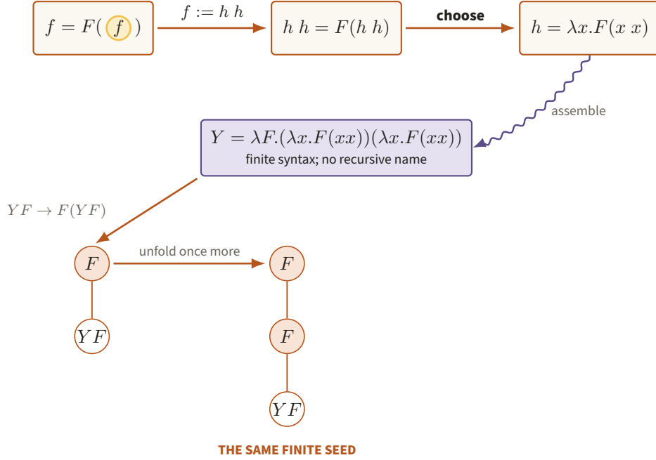
Figure 28. The fixed-point equation is solved by self-application, yielding finite Y syntax whose reduction grows the tree F(YF) , F(F(YF)) , \dots . Recursion is produced by running the seed rather than by storing an infinite or recursively named term.
