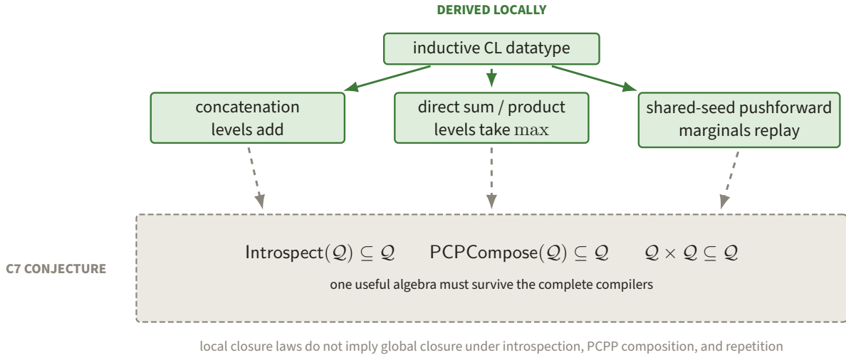
Figure 88. Green branches are closure operations carried by the inductive CL datatype, whereas the dashed slate box is the stronger compiler-wide closure hypothesis C7. The distinction blocks local concatenation and product laws from silently becoming an introspection or compression theorem.
