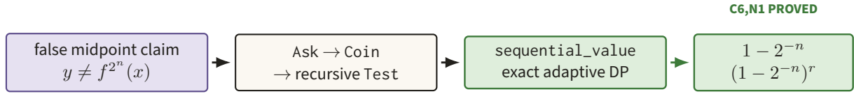
Figure 95. The Ask/Coin/Test recurrence is evaluated by an exact adaptive dynamic program. Its one-copy and sequential-AND values are the proved C6 and N1 formulas, not claims about quantum parallel repetition.
