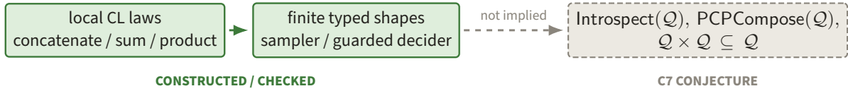
Figure 87. Constructed local CL operations and finite typed shapes stop at the dashed arrow before compiler-wide closure of \mathcal{Q} . That missing implication is precisely the C7 structural conjecture rather than a consequence of the datatype alone.
