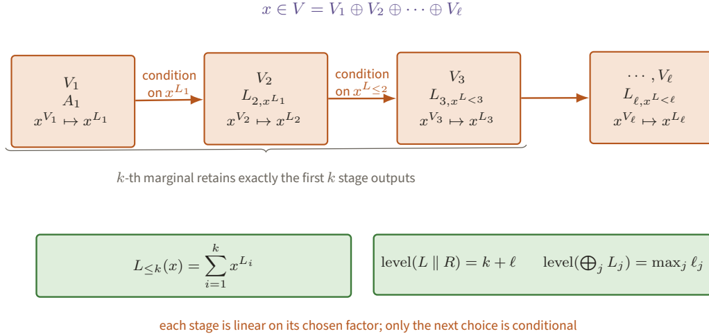
Figure 82. Each rust stage applies a linear map on one complementary register, while the labelled dependency lets earlier outputs select the next stage. Marginals sum prefixes of stage outputs, concatenation adds levels, and direct sum takes their maximum.
