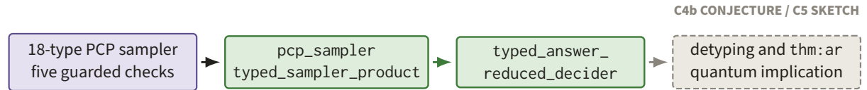
Figure 94. The 18-type sampler and guarded answer-reduced decider have constructed or finite-checked shapes. Detying and the quantum implication in thm:ar remain dashed at C4b CONJECTURE and C5 SKETCH.
