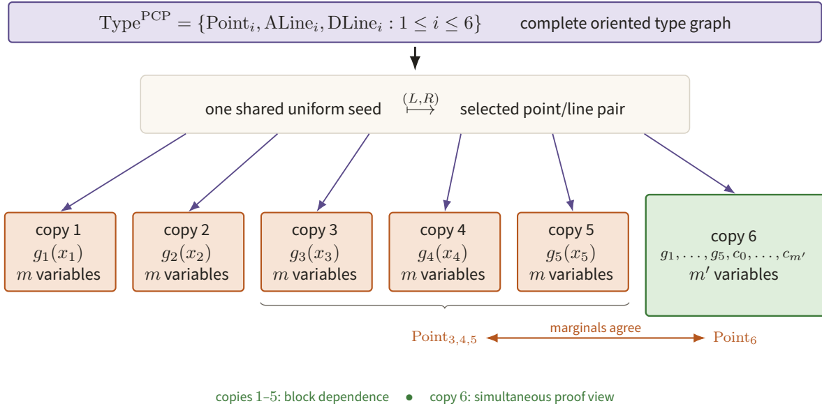
Figure 85. Copies one through five test the five block polynomials individually, while copy six tests the complete (g_1, \dots, g_5, c_0, \dots, c_{m'}) bundle in dimension m' . The 18 point/axis-line/diagonal-line types share one ambient seed and a complete oriented type graph.
