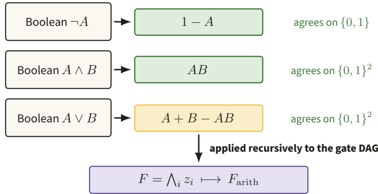
Figure 72. Negation, conjunction, and disjunction become 1 - A , AB , and the amber polynomial A + B - AB , respectively. These replacements preserve values on the Boolean cube while producing the formal polynomial consumed by the PCP layer.
