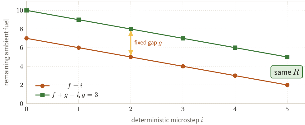
Figure 50. Two runs follow the same charged transitions while their remaining-fuel curves stay exactly g units apart. Once the smaller budget reaches a non-fuel result R , extra fuel cannot change that result.
