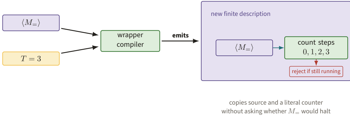
Figure 10. The compiler copies \langle M_{=} \rangle beside a literal three-step counter whose exhausted branch rejects. Producing this bounded wrapper is a terminating syntactic operation and never requires deciding the wrapped machine's unbounded behavior.
