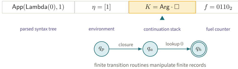
Figure 34. The evaluator’s work tape contains a parsed application, environment, focused continuation frame, and binary fuel counter as four concrete finite regions. Fixed state routines can therefore simulate every charged evaluation rule with polynomial overhead.
