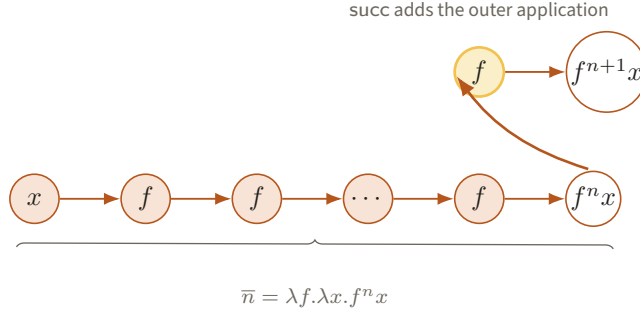
Figure 25. A Church numeral is an n -stage application spine from x to f^n x , and successor adds the amber outer f . The drawing separates representability by iteration from the binary storage used for efficient resource bounds.
