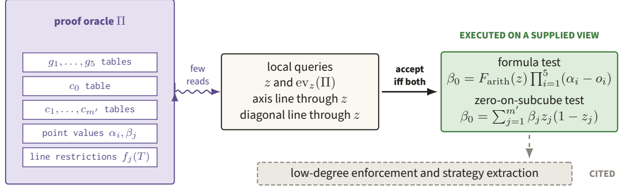
Figure 78. Point and line queries land in evaluation tables for g_1, \dots, g_5, c_0, \dots, c_{m'} , while the green decider checks the two displayed identities at z . Those local checks are executable, but low-degree enforcement and quantum strategy extraction remain cited analytic input.
