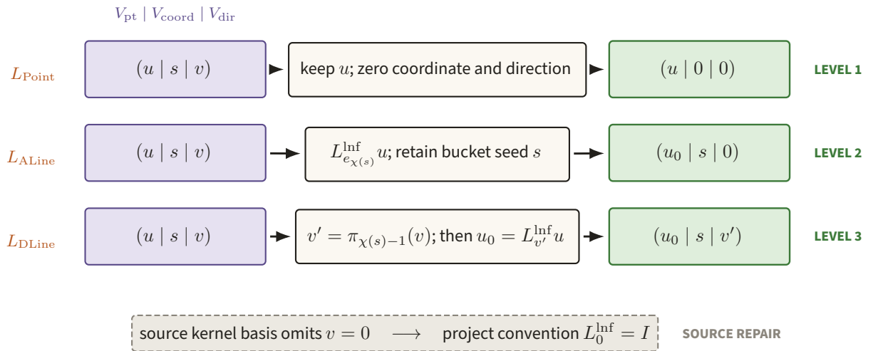
Figure 84. The point, axis-line, and diagonal-line maps act on the same V_{\text{pt}} \oplus V_{\text{coord}} \oplus V_{\text{dir}} seed but retain different register data. Their one-, two-, and three-level factorizations make the sampled geometry CL, with L_0^{\text{lnf}} = I visibly marked as a source repair.
