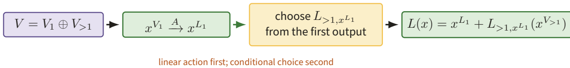
Figure 81. A linear map acts on V_1 , and its actual output selects the continuation on the complementary register V_{>1} . This one-step constructor is the recursive source of every CL level and marginal law below.
