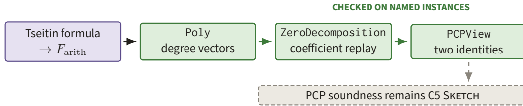
Figure 92. Tseitin syntax flows into sparse polynomials, exact zero-basis division, and the two local PCP identities. Green boxes are checked on named instances, while the separate dashed soundness leaf remains C5 SKETCH.
