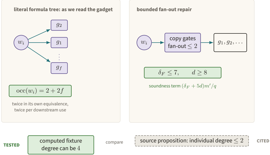
Figure 73. As we read the gate-equivalence formula, a wire used by f later gates contributes 2 + 2f literal occurrences, and the two-gate fixture reaches individual degree four. Bounded fan-out restores the conservative \delta_F \leq 7, d \geq 8 route without conflating a tested account with the cited source proposition.
