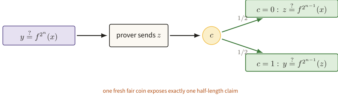
Figure 99. After the prover supplies z , one fresh fair coin selects the left or right half-length orbit claim. This single branching move yields the exact false-claim recurrence behind p_n = 1 - 2^{-n} .
