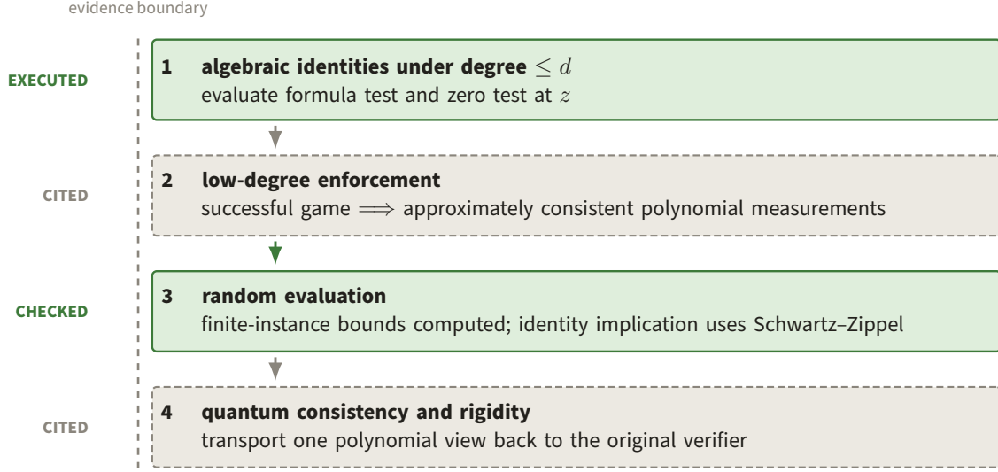
Figure 79. Green strata are computations or finite checks, while dashed slate strata are imported low-degree and quantum implications. The boundary prevents successful local evaluations from being mistaken for a proof of soundness against arbitrary strategies.
