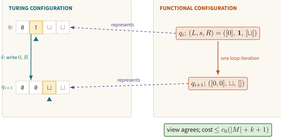
Figure 55. A Turing tape that scans 1 and writes 0 while moving right matches the zipper update from ([0], 1, [\sqcup]) to ([0, 0], \sqcup, []) . This commuting rung is the induction step behind semantic preservation and the c_0(|M| + k + 1) iteration charge.
