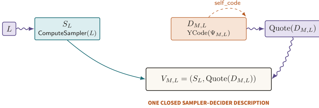
Figure 63. The literal level L produces S_L , while YCode(\Psi_{M,L}) closes its sole self-code socket before quotation places D_{M,L} beside that sampler. The resulting V_{M,L} is one finite normal-form verifier description, not an oracle for either component.
