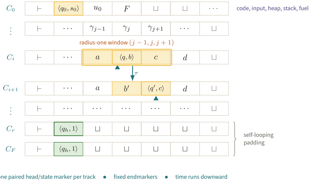
Figure 67. The amber three-cell window in row C_i fixes the marked successor cell and moved head in C_{i+1} . Locality turns a fuel-bounded evaluation into finite constraints, while a halting self-loop supplies exactly F + 1 rows.
