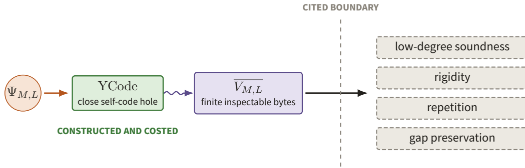
Figure 66. The green path closes \Psi_{M,L} with YCode and emits the finite bytes of \overline{V_{M,L}} , after which the arrow crosses a dashed boundary to low-degree soundness, rigidity, repetition, and gap preservation. Self-reference supplies the program consumed by those theorems; it supplies none of their analytic conclusions.
