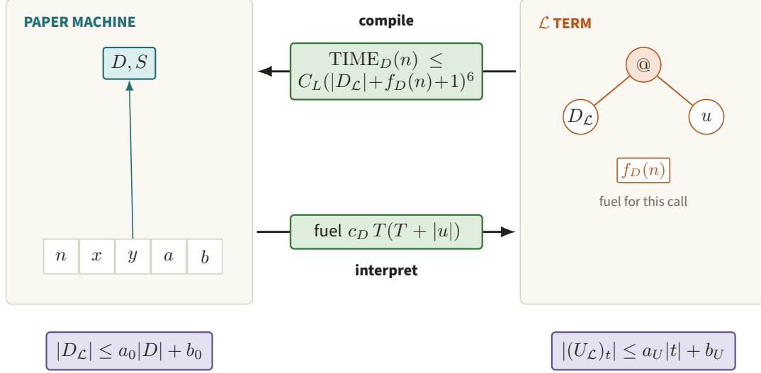
Figure 57. Compiling an \mathcal{L} term incurs the sixth-power Turing bound, while interpreting a T -step machine uses fuel c_D T(T + |u|) ; both source translations remain linear in description size. These explicit arrows are the quantitative content hidden by a bare appeal to Church–Turing equivalence.
