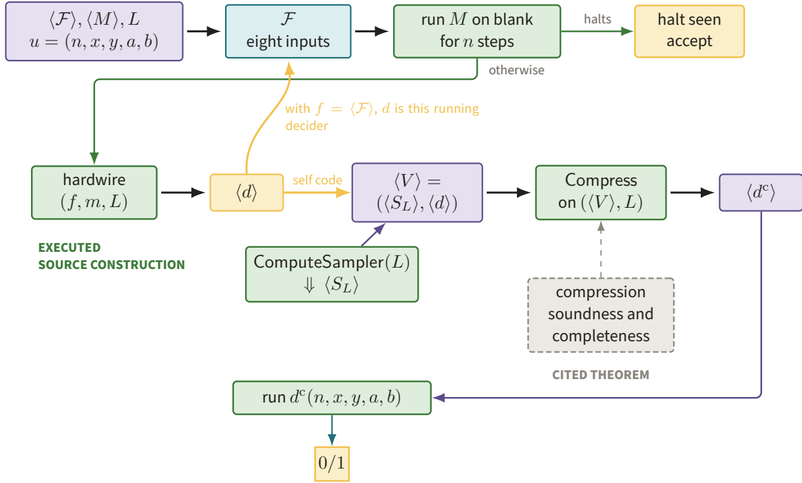
Figure 17. The eight-input machine first accepts a witnessed n -step halt; otherwise it hardwires (f, m, L) , feeds the resulting self-code d into (S_L, d) , compresses, and runs the returned decider. Green boxes are executed source operations while the dashed slate box is the cited game-theoretic guarantee (after fig:halt_f).
