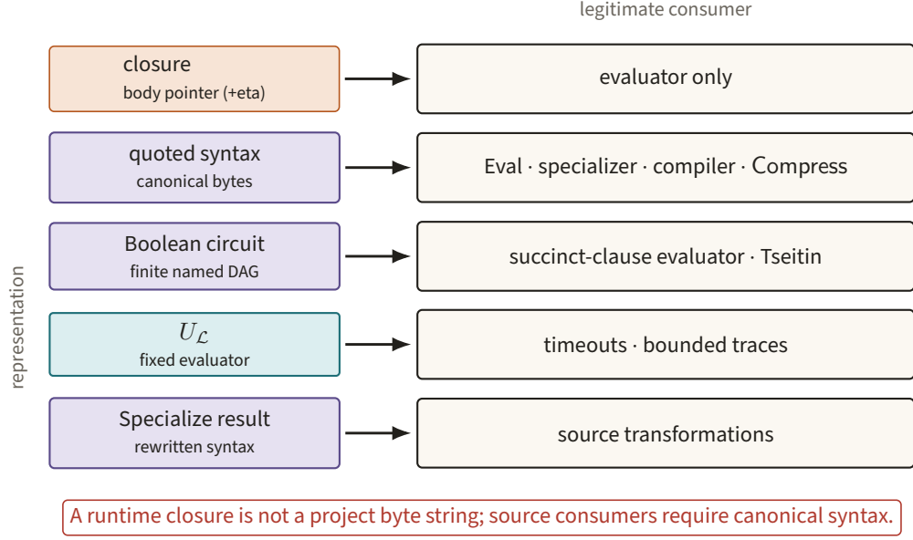
Figure 46. Five representations travel to different legitimate consumers, with canonical quoted syntax occupying the source-code path. Keeping closures off that path prevents runtime sharing from being mistaken for finite description bytes.
