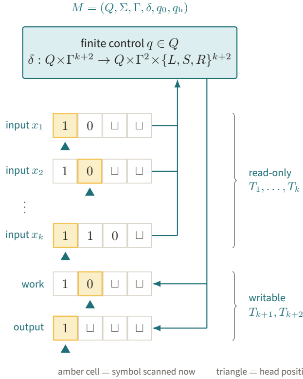
Figure 3. Amber cells are the symbols read by the finite control, with arrows returning updates only to the work and output tapes. This concrete separation of finite rule book from finitely used memory is the machine model simulated throughout the document.
