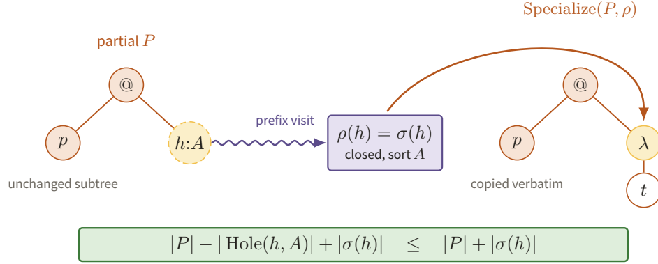
Figure 52. Prefix traversal replaces the unique amber \text{Hole}(h, A) by the closed tree \sigma(h) and copies every other node unchanged. Affineness turns the serialization cost into one deletion plus one insertion, yielding the stated linear size bound.
