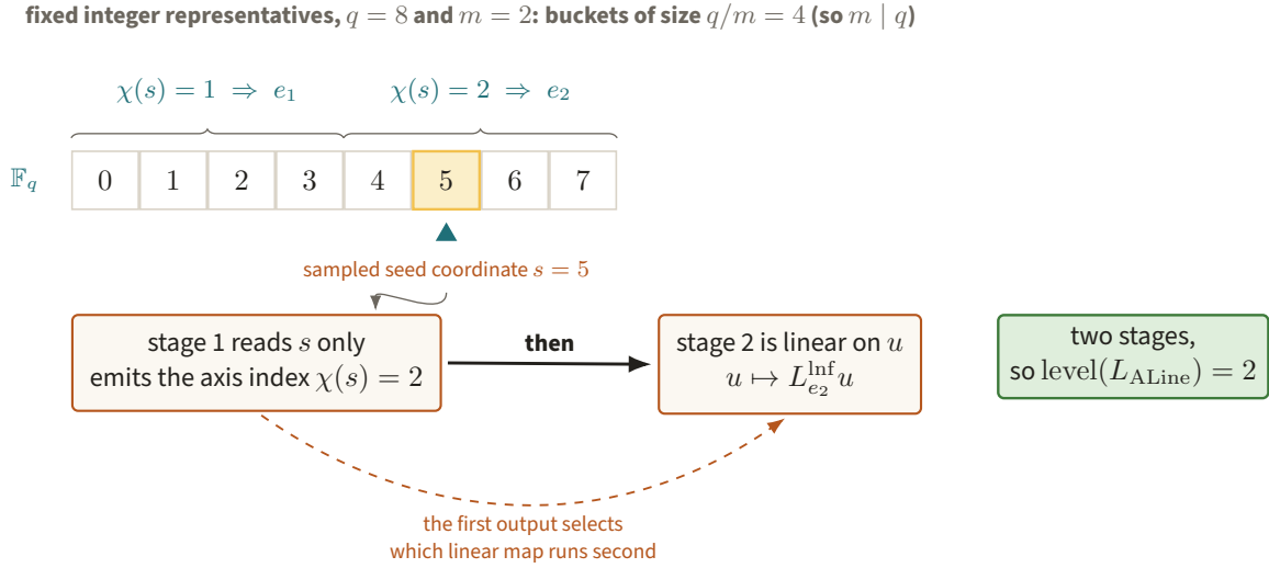
Figure 83. The amber seed coordinate s = 5 falls in the second of the two q/m = 4 -element buckets, so \chi(s) = 2 and the axis-line map takes its direction e_2 from a stage that reads s alone. The second stage is then linear on u with the choice already fixed, which is exactly why L_{\text{ALine}} is conditionally linear of level two rather than one.
