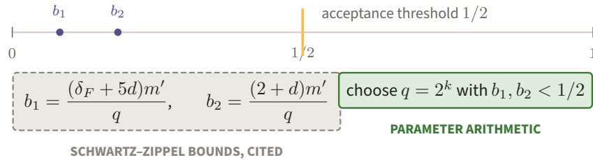
Figure 80. Both Schwartz–Zippel bounds must fall left of the amber acceptance threshold, which is exactly what the choice q = 2^k buys. The two bounds are cited analytic input; only the parameter arithmetic that compares them with 1/2 is executed here.
