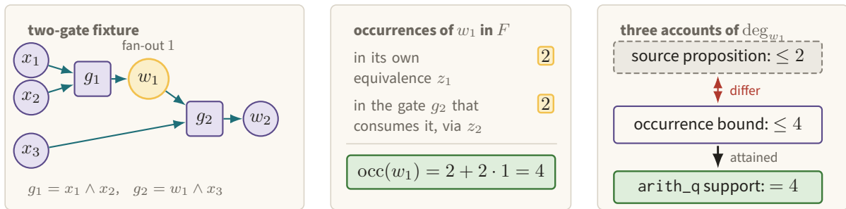
Figure 74. The amber wire w_1 occurs four times in the literal formula tree and the measured sparse-support degree meets that bound, while the cited proposition allows two; our reading of the gadget may be the thing at fault (finding F1 of docs/findings.md).
