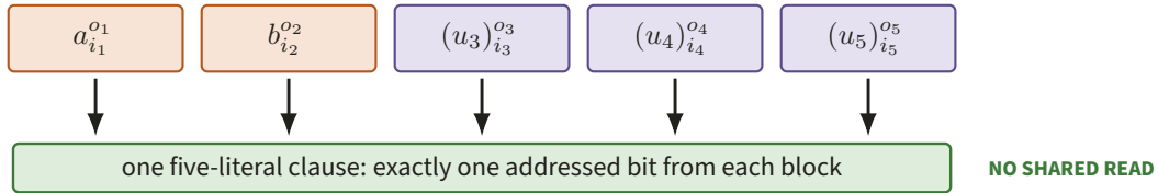
Figure 71. A decoupled clause reads exactly one addressed literal from each of a, b, u_3, u_4, u_5 , with the two answer blocks distinguished in rust. Independent low-degree answers can now supply the five locations without pretending to be three reads of one shared assignment.
