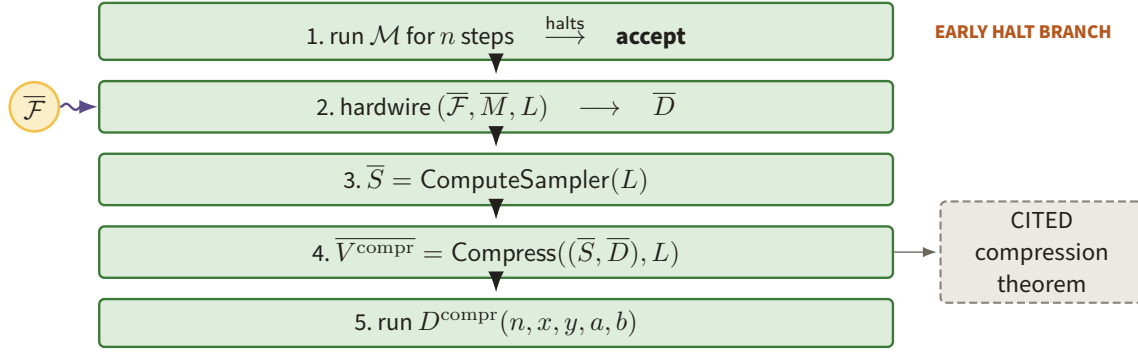
Figure 62. The machine \mathcal{F} first takes the amber early-halt branch or else hardwires its own description, computes S_L , calls \text{Compress} , and runs the returned decider (after fig:halt_f ). The dashed box isolates the cited compression guarantee from the green source operations that are actually performed.
