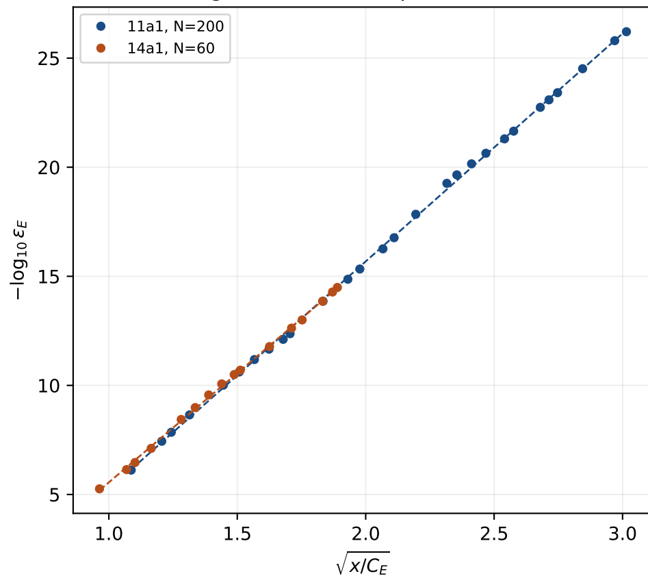
Straight-line fit in the predicted scale
