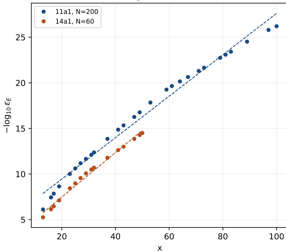
Straight-line fit in x
