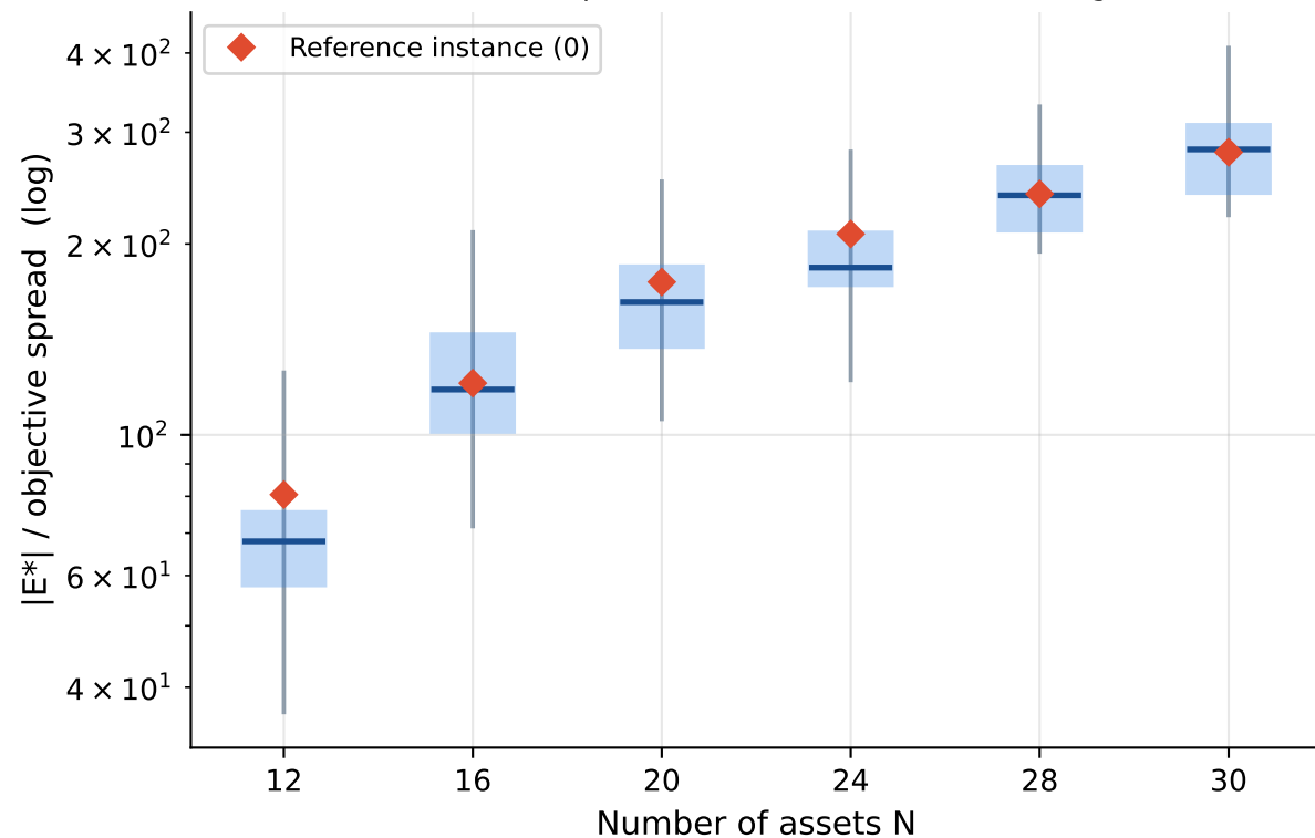
How far the gap denominator overstates the objective (30 instances per size; box = IQR, whisker = range)
