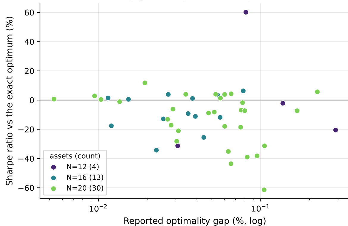
Every sub-optimal QAOA solution in the instance sweep (the gap does not predict the Sharpe loss)
