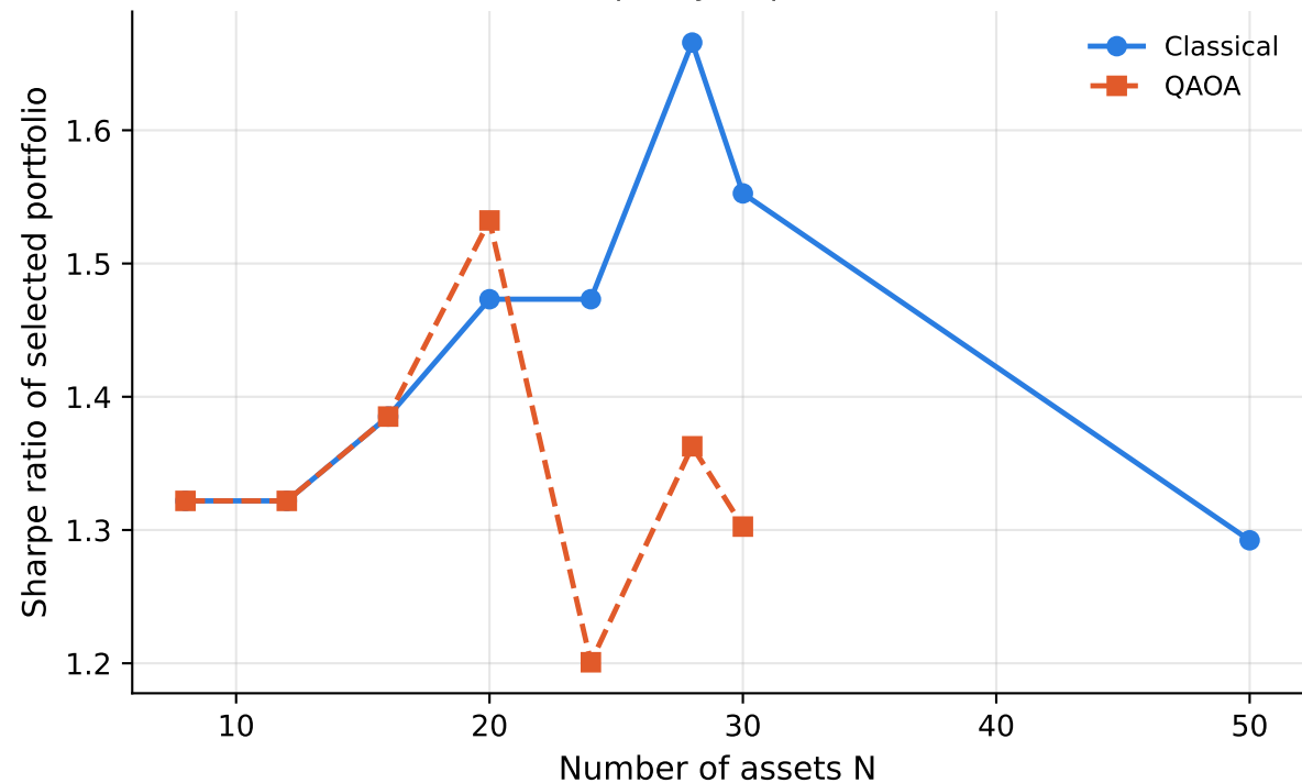
Portfolio quality vs problem size
